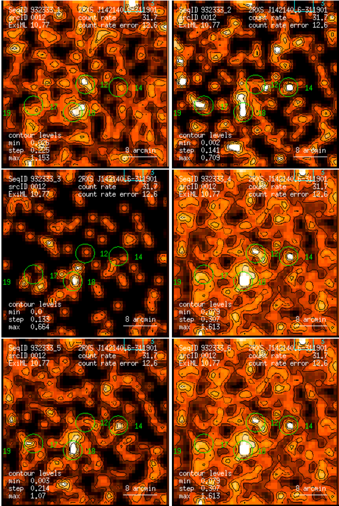
Figure 12: RASS 932333: detection 0012: band rate images, Gaussian filter: (1) PSPC channels 11 – 41, (2) 52 – 90, (3) 91 – 201, (4) 11 – 235, (5) 52 – 201, (6) 11 – 201. Broad band rates in counts/ks. Band rate contour levels in counts/ks/arcmin 2 .
