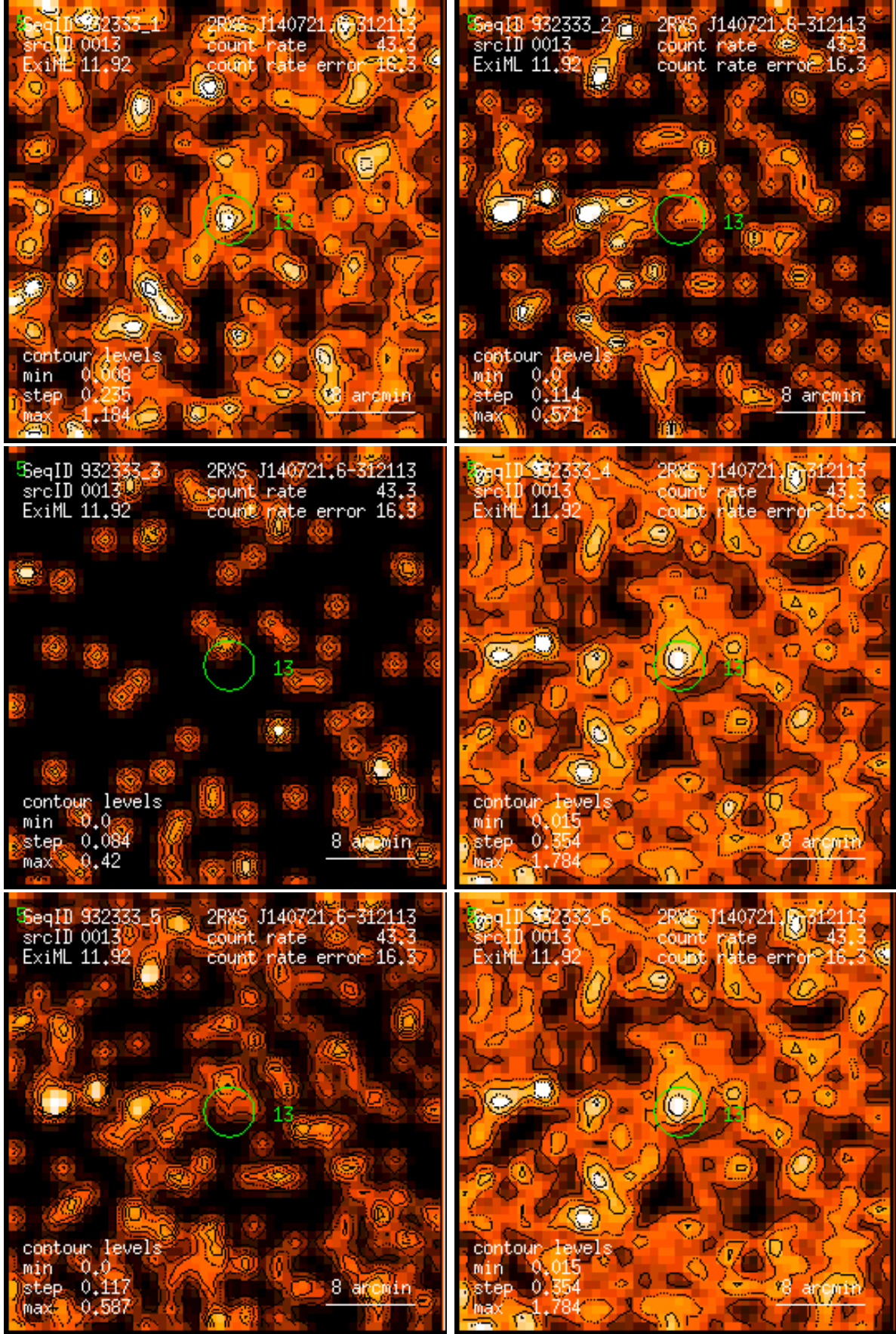
Figure 13: RASS 932333: detection 0013: band rate images, Gaussian filter: (1) PSPC channels 11 – 41, (2) 52 – 90, (3) 91 – 201, (4) 11 – 235, (5) 52 – 201, (6) 11 – 201. Broad band rates in counts/ks. Band rate contour levels in counts/ks/arcmin 2 .
