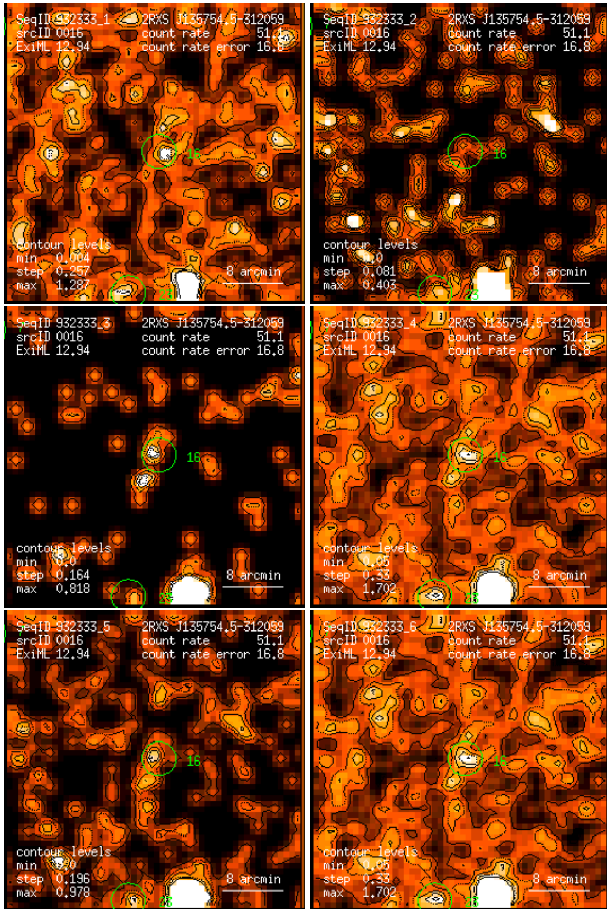
Figure 16: RASS 932333: detection 0016: band rate images, Gaussian filter: (1) PSPC channels 11 – 41, (2) 52 – 90, (3) 91 – 201, (4) 11 – 235, (5) 52 – 201, (6) 11 – 201. Broad band rates in counts/ks. Band rate contour levels in counts/ks/arcmin 2 .
