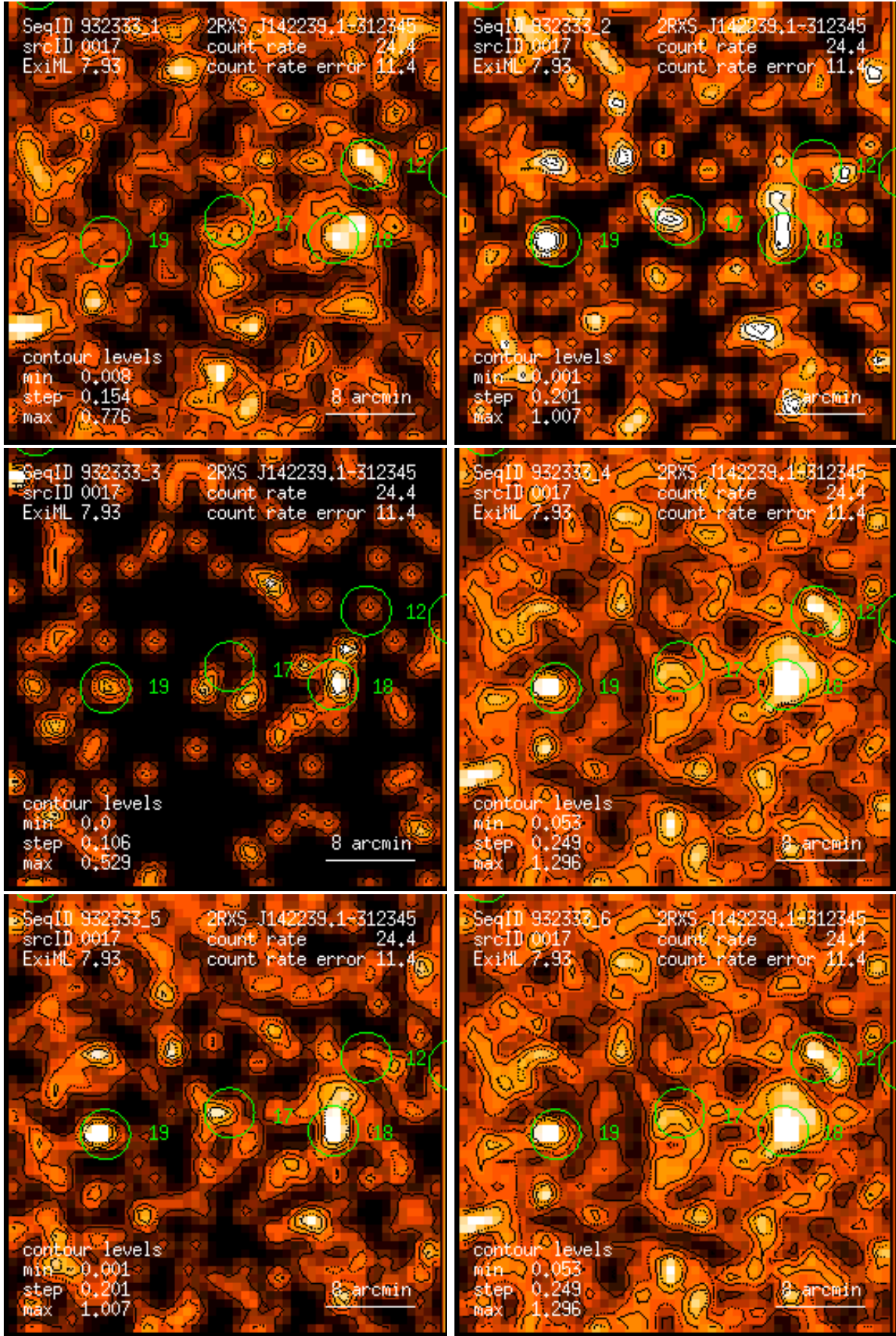
Figure 17: RASS 932333: detection 0017: band rate images, Gaussian filter: (1) PSPC channels 11 – 41, (2) 52 – 90, (3) 91 – 201, (4) 11 – 235, (5) 52 – 201, (6) 11 – 201. Broad band rates in counts/ks. Band rate contour levels in counts/ks/arcmin 2 .
