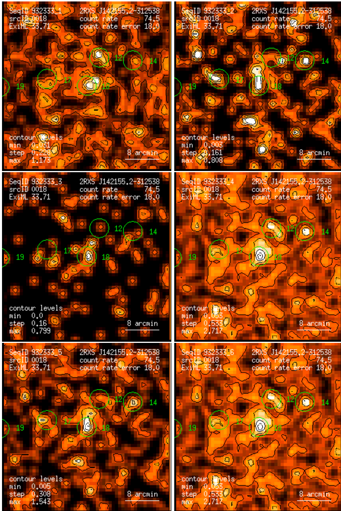
Figure 18: RASS 932333: detection 0018: band rate images, Gaussian filter: (1) PSPC channels 11 – 41, (2) 52 – 90, (3) 91 – 201, (4) 11 – 235, (5) 52 – 201, (6) 11 – 201. Broad band rates in counts/ks. Band rate contour levels in counts/ks/arcmin 2 .
