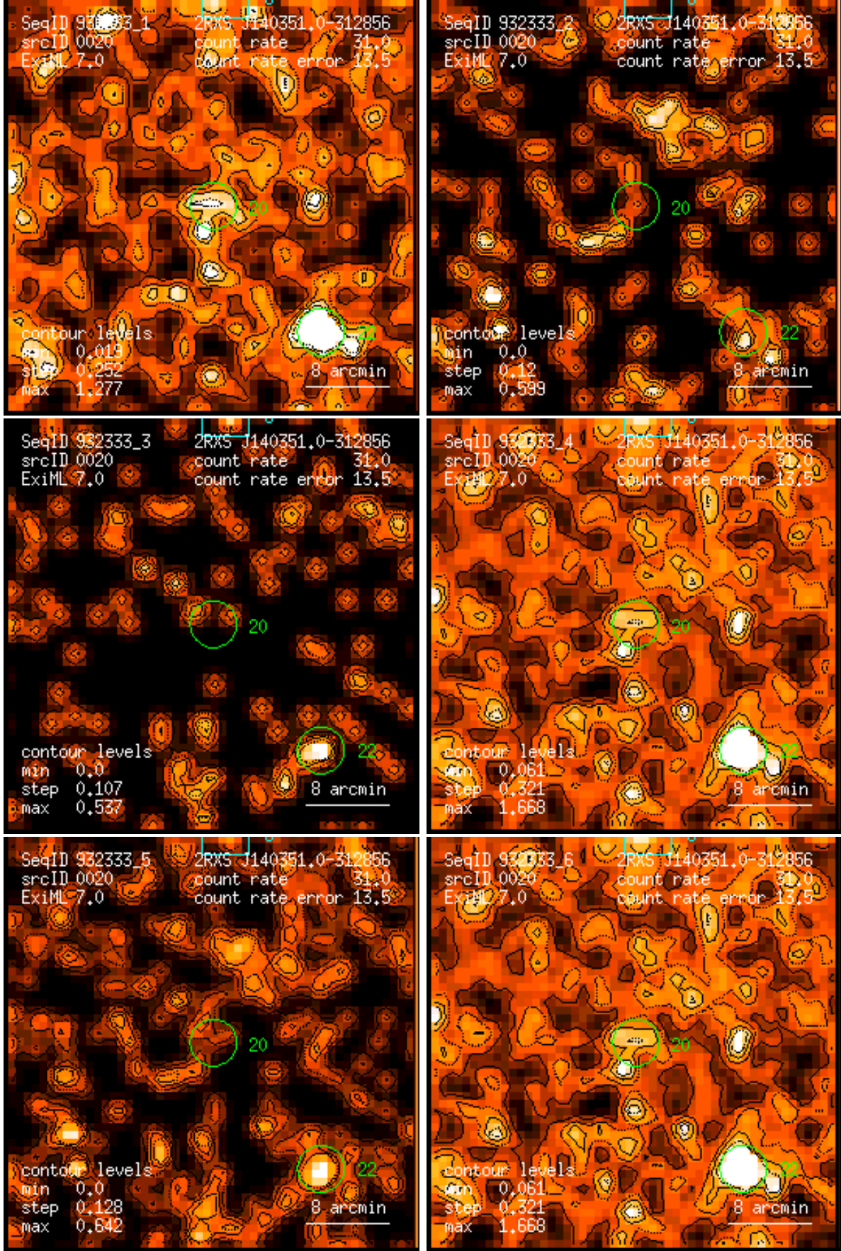
Figure 20: RASS 932333: detection 0020: band rate images, Gaussian filter: (1) PSPC channels 11 – 41, (2) 52 – 90, (3) 91 – 201, (4) 11 – 235, (5) 52 – 201, (6) 11 – 201. Broad band rates in counts/ks. Band rate contour levels in counts/ks/arcmin 2 .
