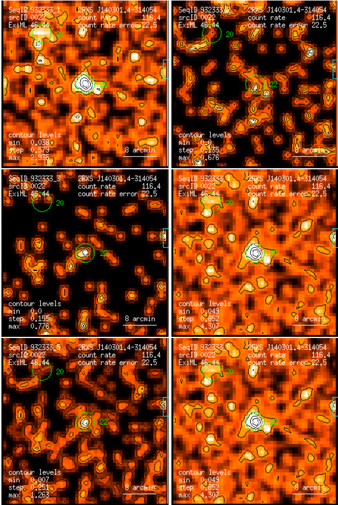
Figure 22: RASS 932333: detection 0022: band rate images, Gaussian filter: (1) PSPC channels 11 – 41, (2) 52 – 90, (3) 91 – 201, (4) 11 – 235, (5) 52 – 201, (6) 11 – 201. Broad band rates in counts/ks. Band rate contour levels in counts/ks/arcmin 2 .
