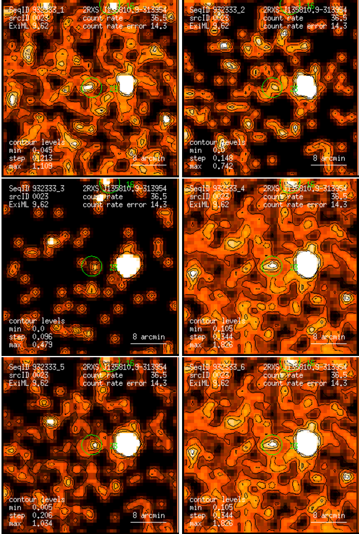
Figure 23: RASS 932333: detection 0023: band rate images, Gaussian filter: (1) PSPC channels 11 – 41, (2) 52 – 90, (3) 91 – 201, (4) 11 – 235, (5) 52 – 201, (6) 11 – 201. Broad band rates in counts/ks. Band rate contour levels in counts/ks/arcmin 2 .
