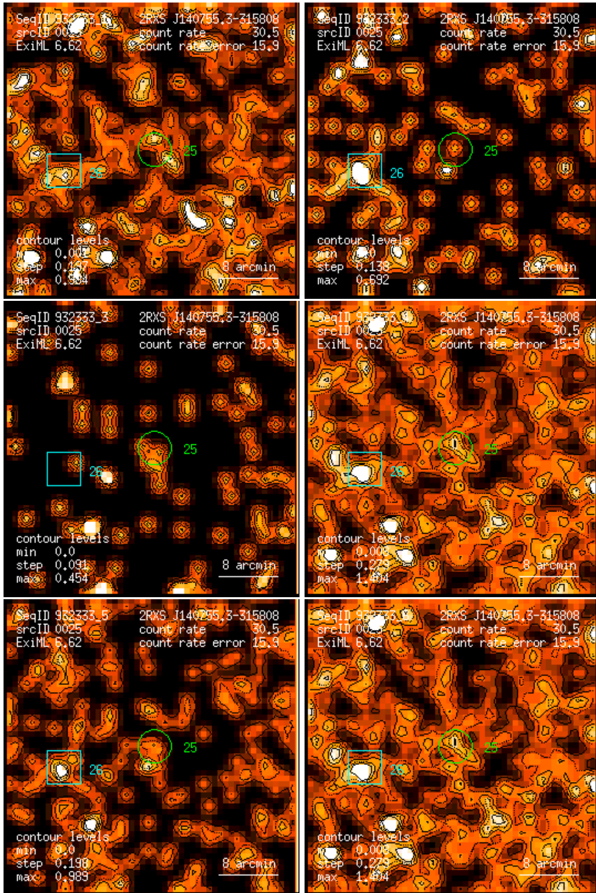
Figure 25: RASS 932333: detection 0025: band rate images, Gaussian filter: (1) PSPC channels 11 – 41, (2) 52 – 90, (3) 91 – 201, (4) 11 – 235, (5) 52 – 201, (6) 11 – 201. Broad band rates in counts/ks. Band rate contour levels in counts/ks/arcmin 2 .
