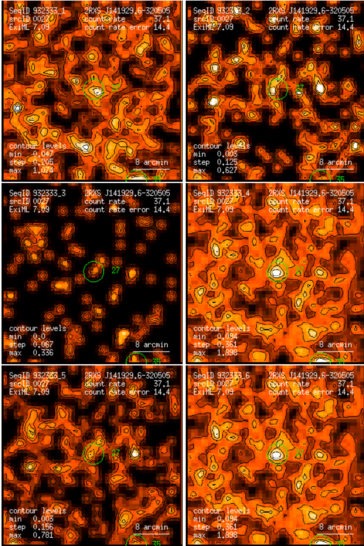
Figure 27: RASS 932333: detection 0027: band rate images, Gaussian filter: (1) PSPC channels 11 – 41, (2) 52 – 90, (3) 91 – 201, (4) 11 – 235, (5) 52 – 201, (6) 11 – 201. Broad band rates in counts/ks. Band rate contour levels in counts/ks/arcmin 2 .
