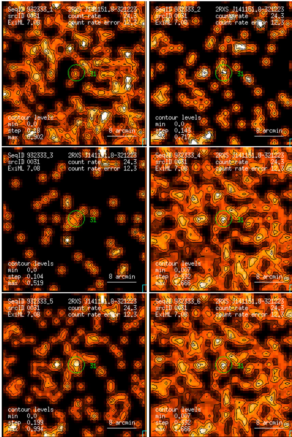
Figure 31: RASS 932333: detection 0031: band rate images, Gaussian filter: (1) PSPC channels 11 – 41, (2) 52 – 90, (3) 91 – 201, (4) 11 – 235, (5) 52 – 201, (6) 11 – 201. Broad band rates in counts/ks. Band rate contour levels in counts/ks/arcmin 2 .
