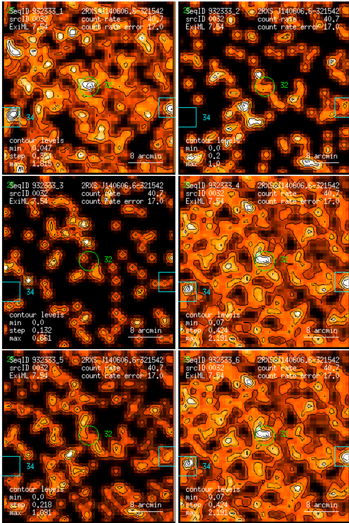
Figure 32: RASS 932333: detection 0032: band rate images, Gaussian filter: (1) PSPC channels 11 – 41, (2) 52 – 90, (3) 91 – 201, (4) 11 – 235, (5) 52 – 201, (6) 11 – 201. Broad band rates in counts/ks. Band rate contour levels in counts/ks/arcmin 2 .
