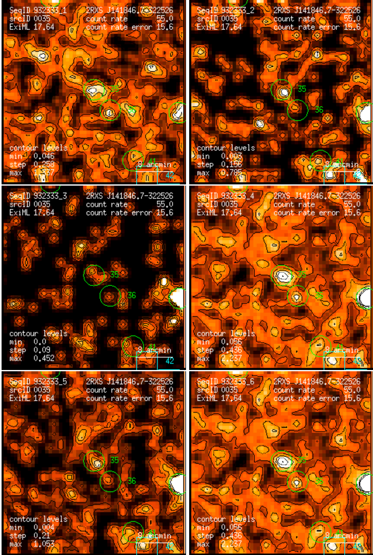
Figure 35: RASS 932333: detection 0035: band rate images, Gaussian filter: (1) PSPC channels 11 – 41, (2) 52 – 90, (3) 91 – 201, (4) 11 – 235, (5) 52 – 201, (6) 11 – 201. Broad band rates in counts/ks. Band rate contour levels in counts/ks/arcmin 2 .
