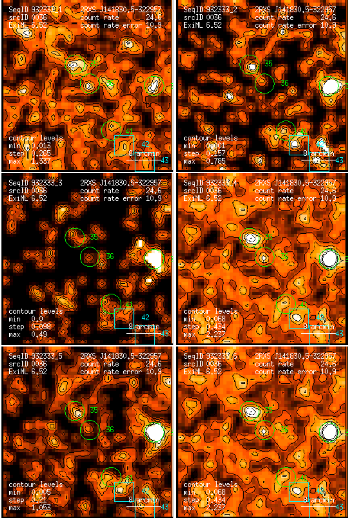
Figure 36: RASS 932333: detection 0036: band rate images, Gaussian filter: (1) PSPC channels 11 – 41, (2) 52 – 90, (3) 91 – 201, (4) 11 – 235, (5) 52 – 201, (6) 11 – 201. Broad band rates in counts/ks. Band rate contour levels in counts/ks/arcmin 2 .
