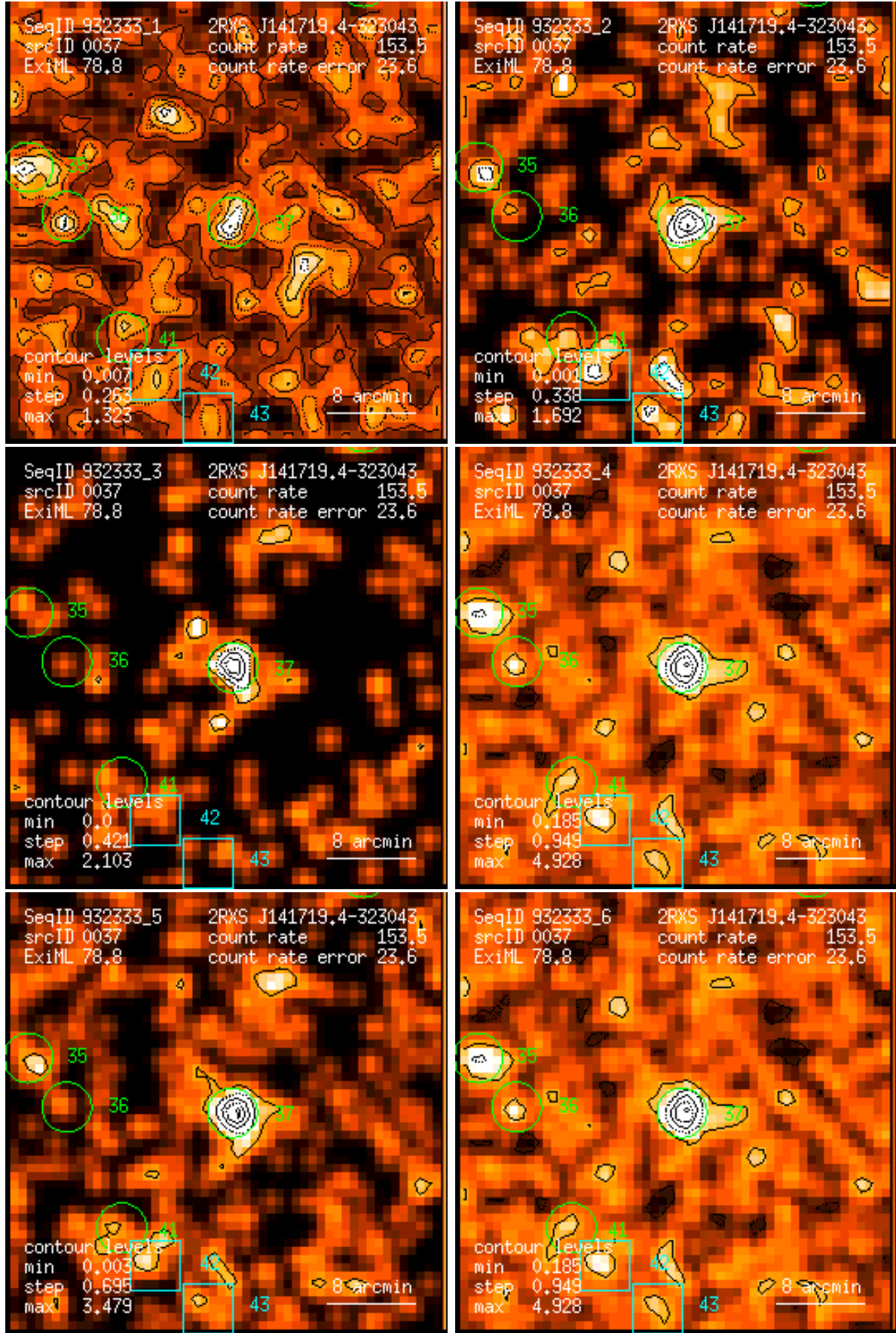
Figure 37: RASS 932333: detection 0037: band rate images, Gaussian filter: (1) PSPC channels 11 – 41, (2) 52 – 90, (3) 91 – 201, (4) 11 – 235, (5) 52 – 201, (6) 11 – 201. Broad band rates in counts/ks. Band rate contour levels in counts/ks/arcmin 2 .
