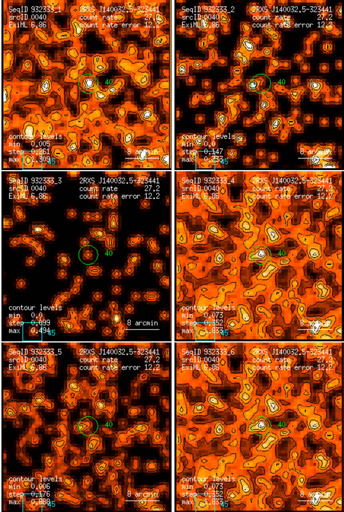
Figure 40: RASS 932333: detection 0040: band rate images, Gaussian filter: (1) PSPC channels 11 – 41, (2) 52 – 90, (3) 91 – 201, (4) 11 – 235, (5) 52 – 201, (6) 11 – 201. Broad band rates in counts/ks. Band rate contour levels in counts/ks/arcmin 2 .
