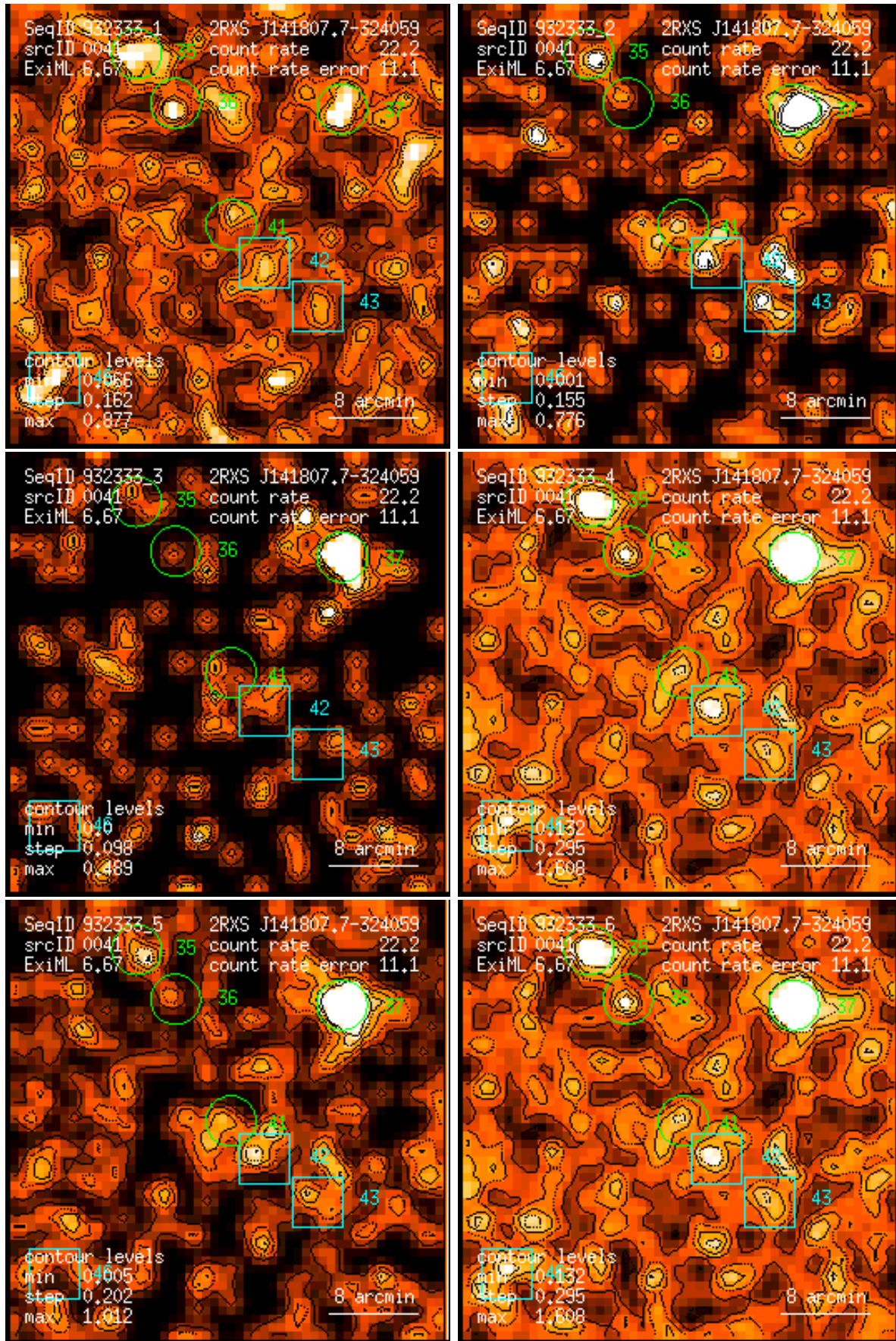
Figure 41: RASS 932333: detection 0041: band rate images, Gaussian filter: (1) PSPC channels 11 – 41, (2) 52 – 90, (3) 91 – 201, (4) 11 – 235, (5) 52 – 201, (6) 11 – 201. Broad band rates in counts/ks. Band rate contour levels in counts/ks/arcmin 2 .
