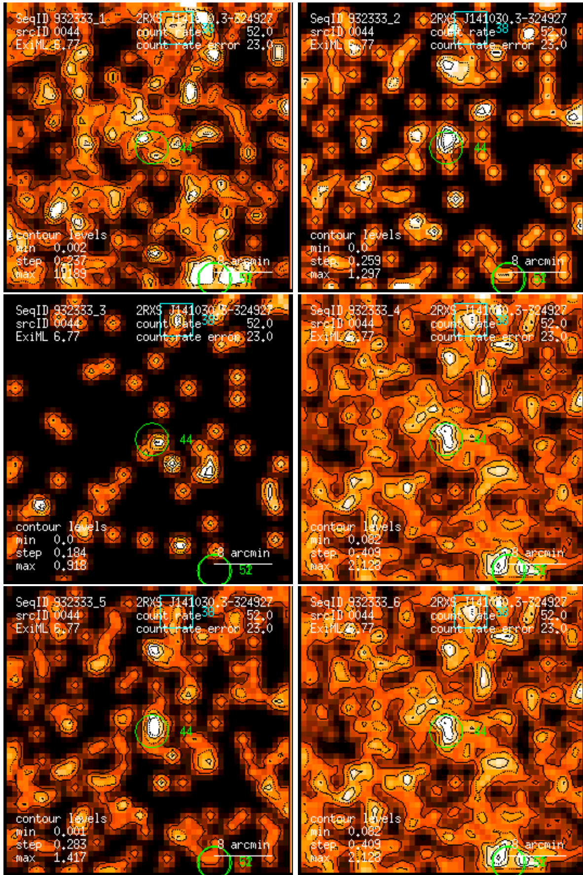
Figure 44: RASS 932333: detection 0044: band rate images, Gaussian filter: (1) PSPC channels 11 – 41, (2) 52 – 90, (3) 91 – 201, (4) 11 – 235, (5) 52 – 201, (6) 11 – 201. Broad band rates in counts/ks. Band rate contour levels in counts/ks/arcmin 2 .
