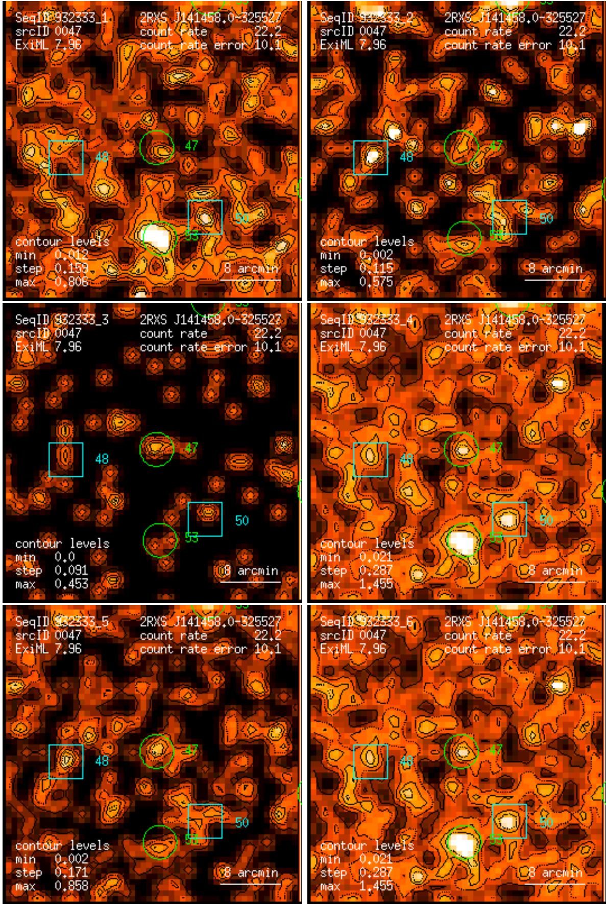
Figure 47: RASS 932333: detection 0047: band rate images, Gaussian filter: (1) PSPC channels 11 – 41, (2) 52 – 90, (3) 91 – 201, (4) 11 – 235, (5) 52 – 201, (6) 11 – 201. Broad band rates in counts/ks. Band rate contour levels in counts/ks/arcmin 2 .
