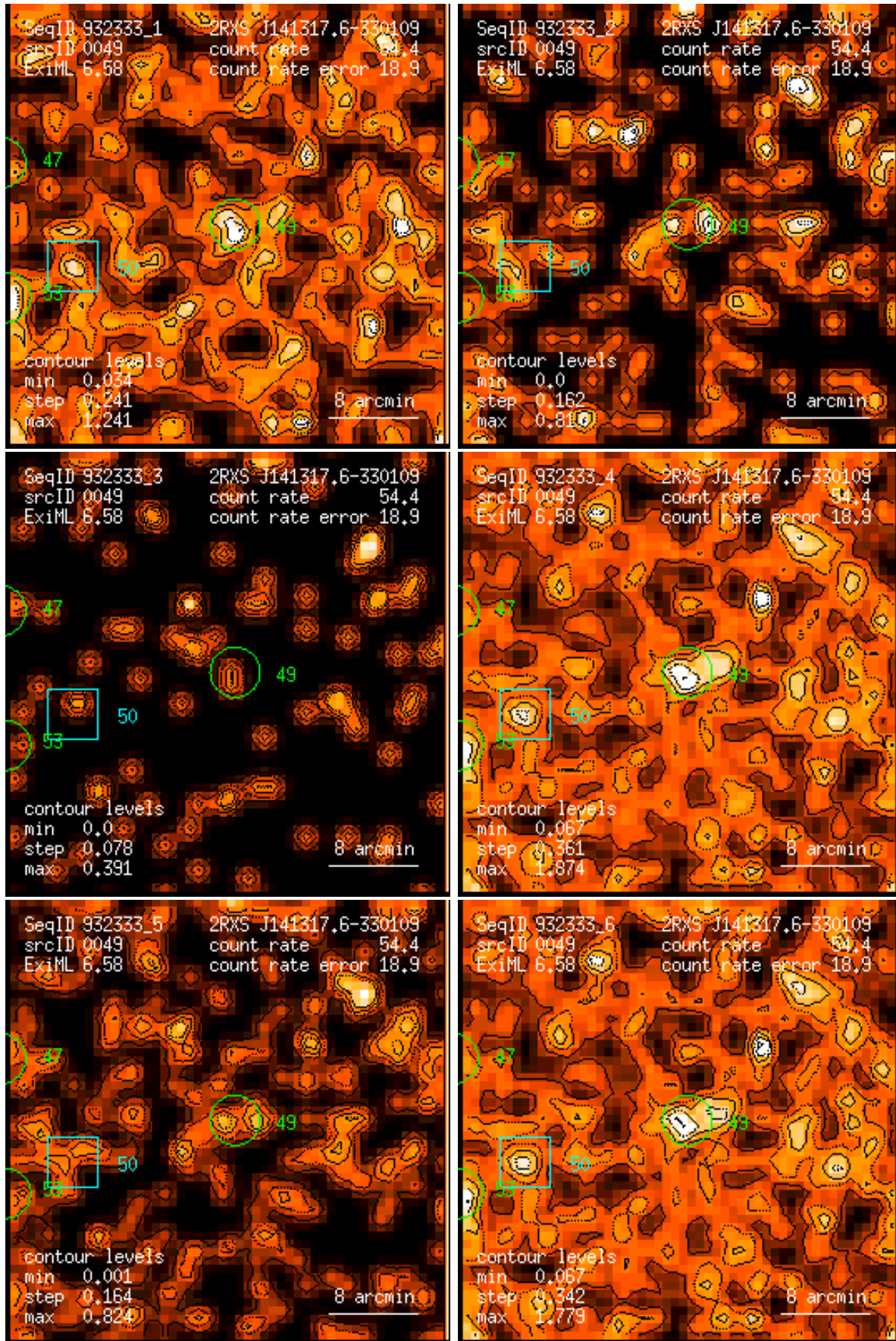
Figure 49: RASS 932333: detection 0049: band rate images, Gaussian filter: (1) PSPC channels 11 – 41, (2) 52 – 90, (3) 91 – 201, (4) 11 – 235, (5) 52 – 201, (6) 11 – 201. Broad band rates in counts/ks. Band rate contour levels in counts/ks/arcmin 2 .
