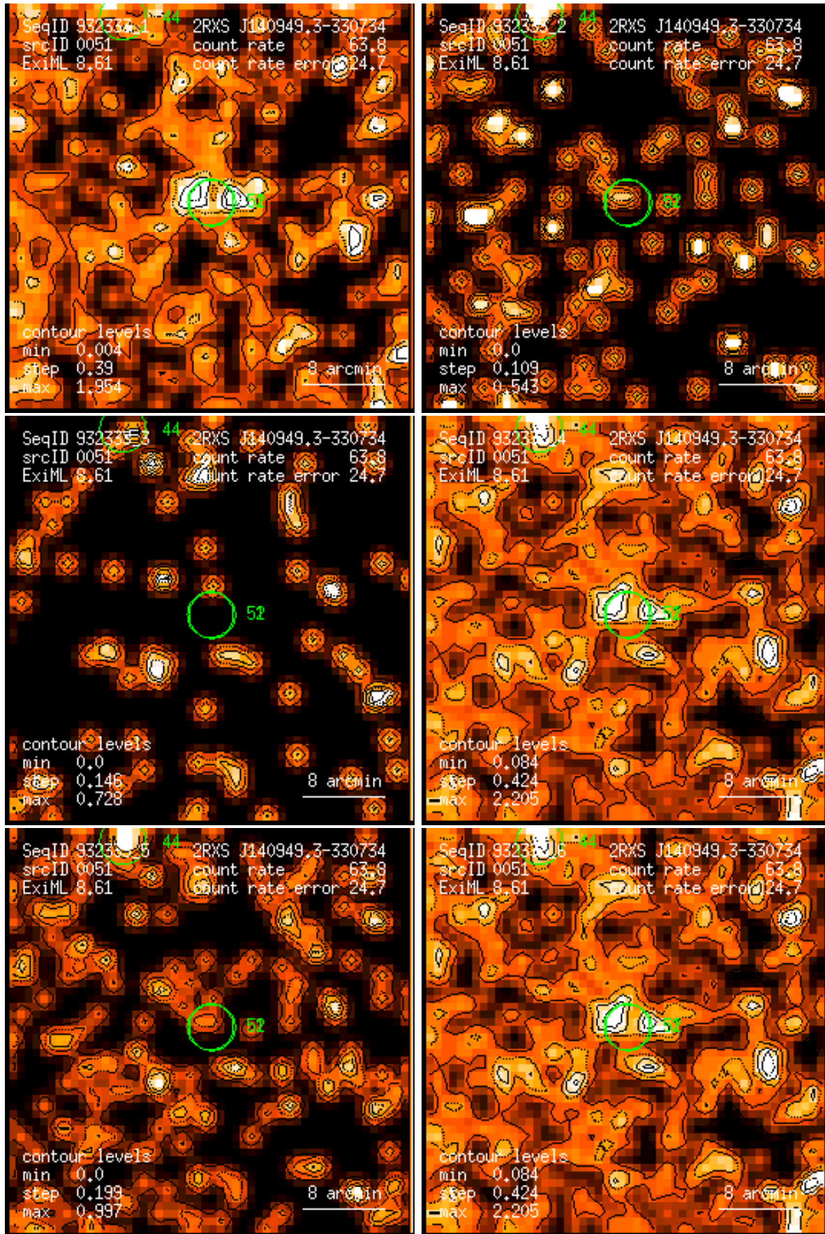
Figure 51: RASS 932333: detection 0051: band rate images, Gaussian filter: (1) PSPC channels 11 – 41, (2) 52 – 90, (3) 91 – 201, (4) 11 – 235, (5) 52 – 201, (6) 11 – 201. Broad band rates in counts/ks. Band rate contour levels in counts/ks/arcmin 2 .
