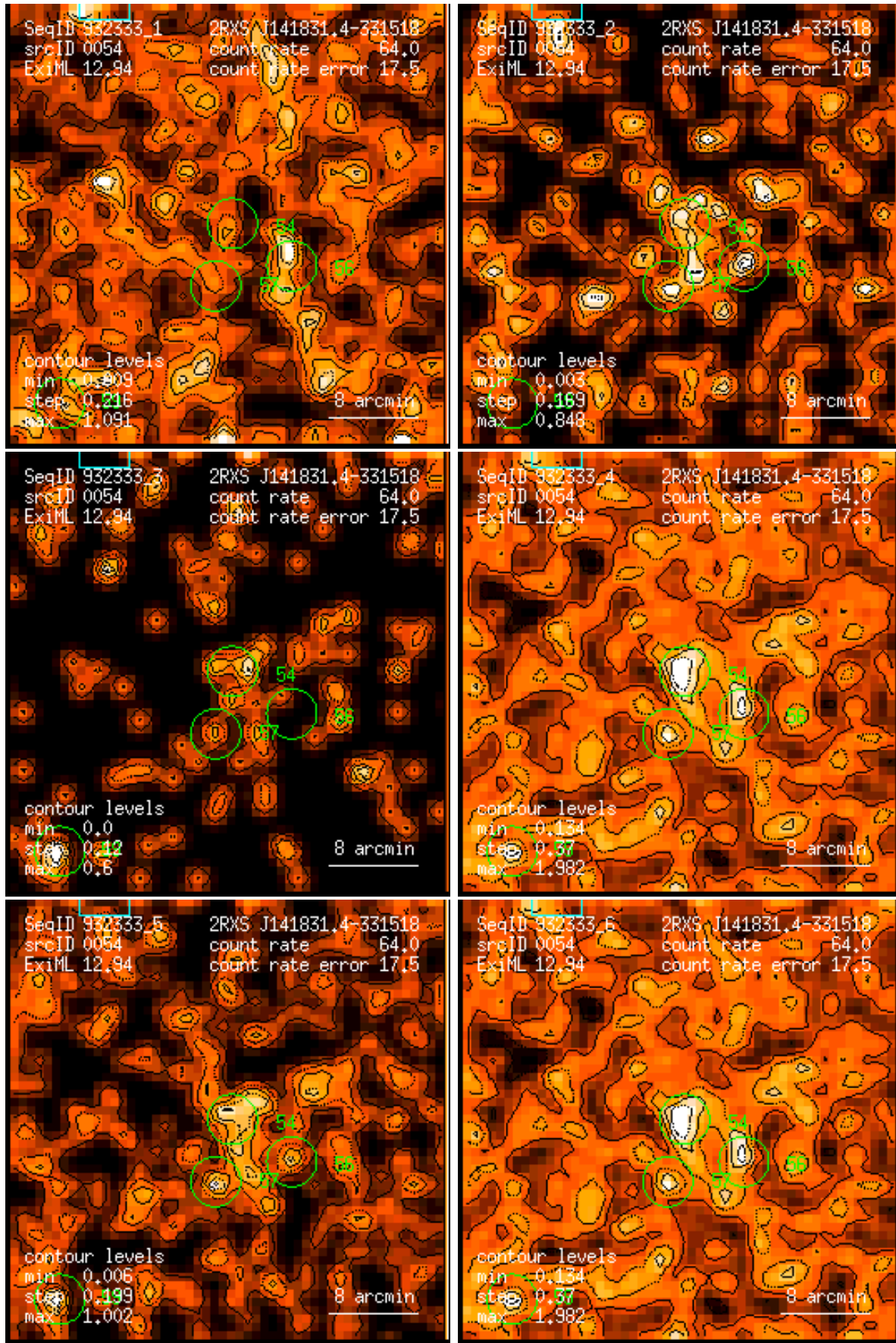
Figure 54: RASS 932333: detection 0054: band rate images, Gaussian filter: (1) PSPC channels 11 – 41, (2) 52 – 90, (3) 91 – 201, (4) 11 – 235, (5) 52 – 201, (6) 11 – 201. Broad band rates in counts/ks. Band rate contour levels in counts/ks/arcmin 2 .
