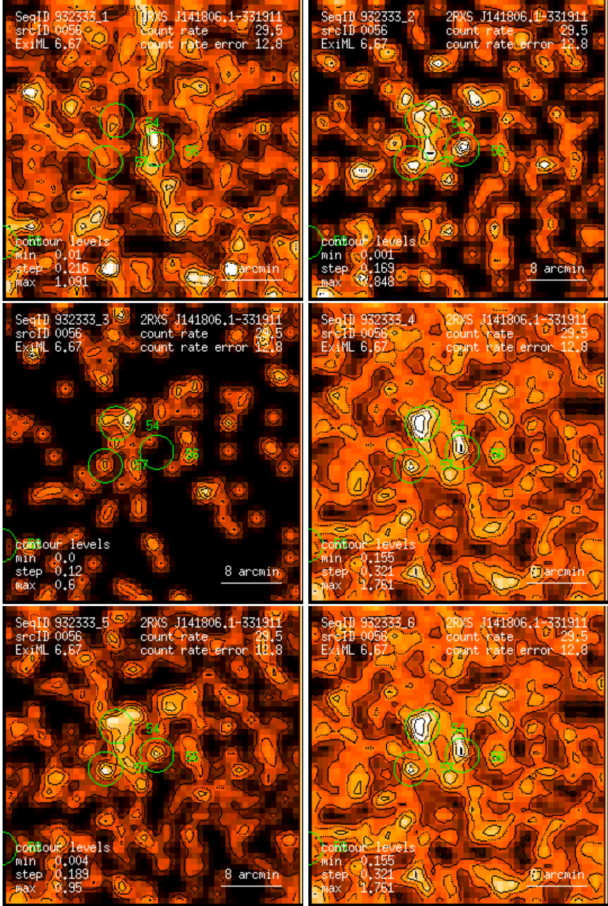
Figure 56: RASS 932333: detection 0056: band rate images, Gaussian filter: (1) PSPC channels 11 – 41, (2) 52 – 90, (3) 91 – 201, (4) 11 – 235, (5) 52 – 201, (6) 11 – 201. Broad band rates in counts/ks. Band rate contour levels in counts/ks/arcmin 2 .
