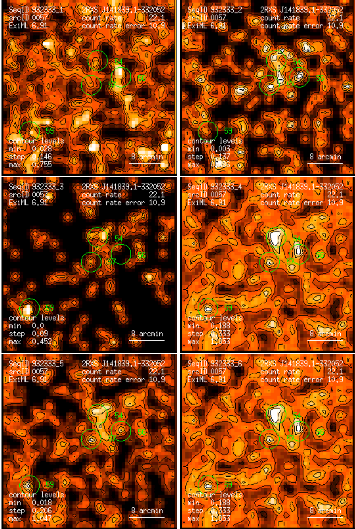
Figure 57: RASS 932333: detection 0057: band rate images, Gaussian filter: (1) PSPC channels 11 – 41, (2) 52 – 90, (3) 91 – 201, (4) 11 – 235, (5) 52 – 201, (6) 11 – 201. Broad band rates in counts/ks. Band rate contour levels in counts/ks/arcmin 2 .
