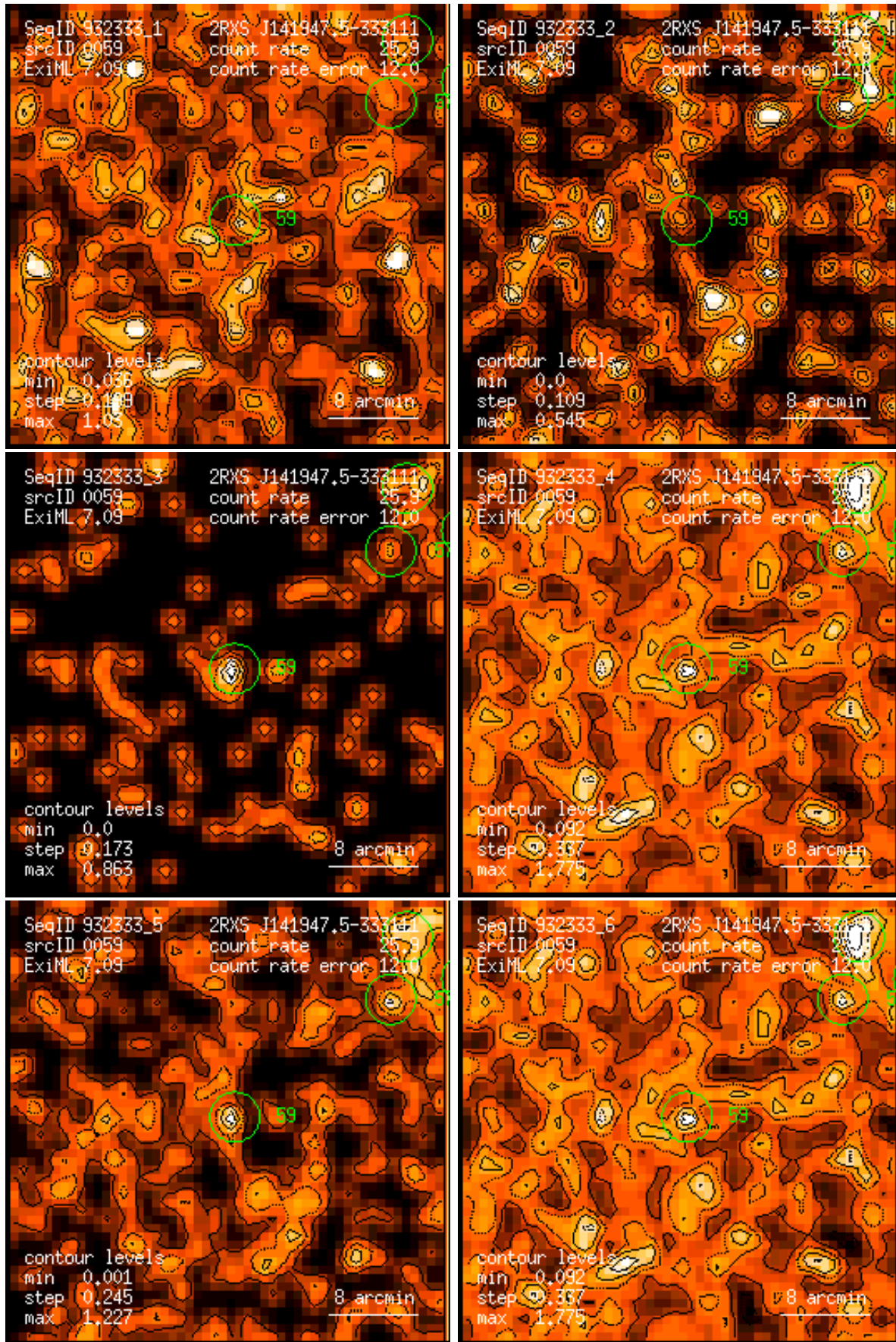
Figure 59: RASS 932333: detection 0059: band rate images, Gaussian filter: (1) PSPC channels 11 – 41, (2) 52 – 90, (3) 91 – 201, (4) 11 – 235, (5) 52 – 201, (6) 11 – 201. Broad band rates in counts/ks. Band rate contour levels in counts/ks/arcmin 2 .
