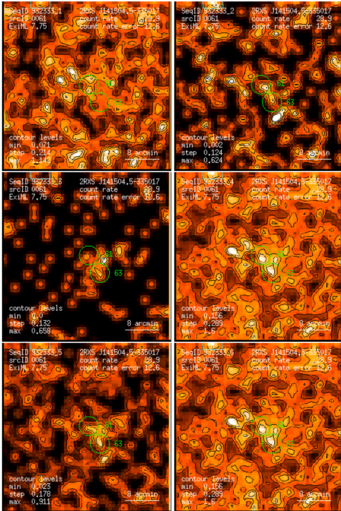
Figure 61: RASS 932333: detection 0061: band rate images, Gaussian filter: (1) PSPC channels 11 – 41, (2) 52 – 90, (3) 91 – 201, (4) 11 – 235, (5) 52 – 201, (6) 11 – 201. Broad band rates in counts/ks. Band rate contour levels in counts/ks/arcmin 2 .
