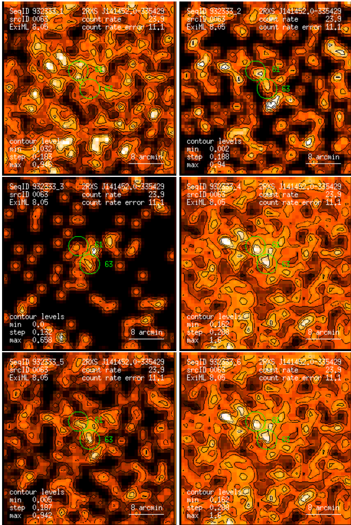
Figure 63: RASS 932333: detection 0063: band rate images, Gaussian filter: (1) PSPC channels 11 – 41, (2) 52 – 90, (3) 91 – 201, (4) 11 – 235, (5) 52 – 201, (6) 11 – 201. Broad band rates in counts/ks. Band rate contour levels in counts/ks/arcmin 2 .
