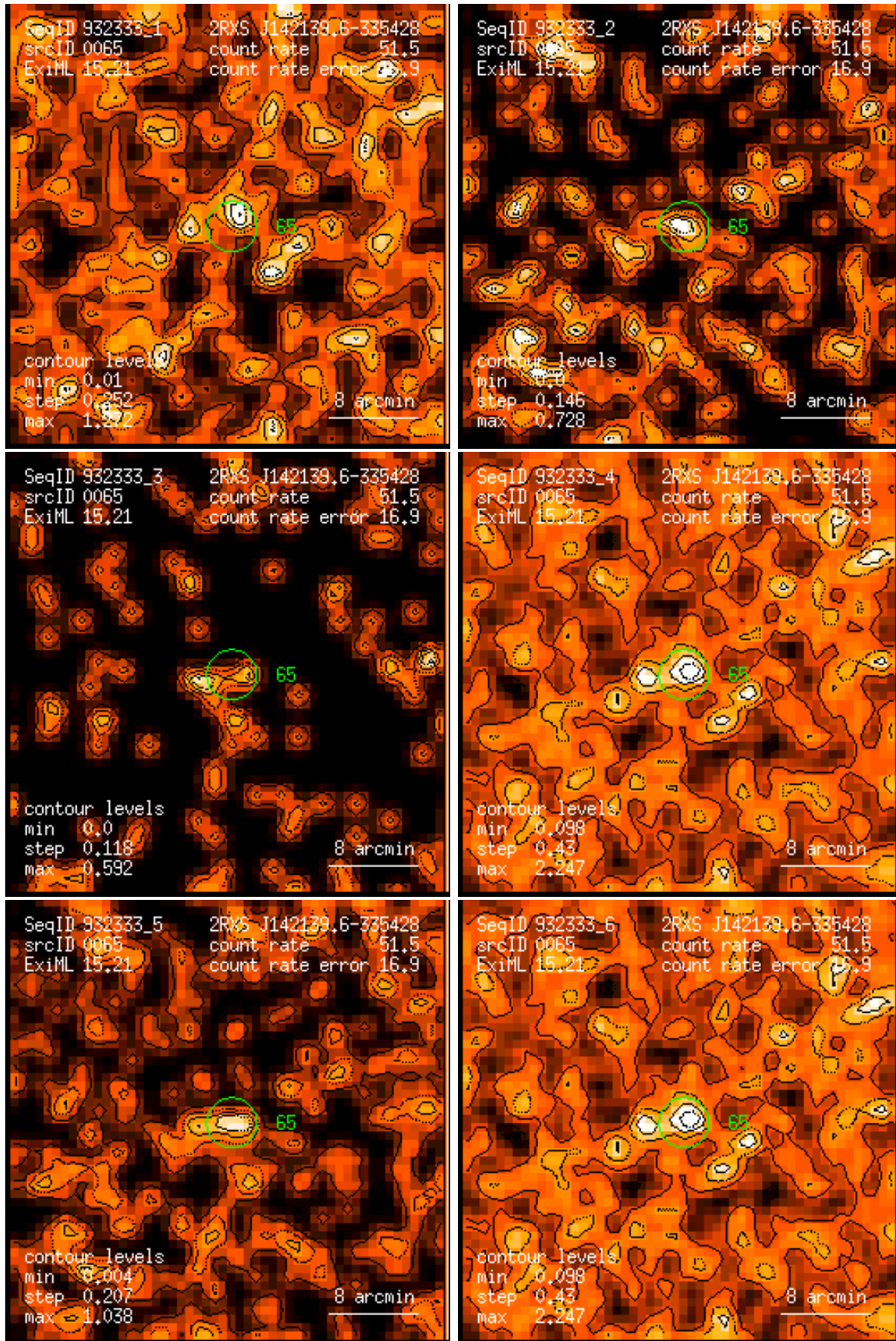
Figure 65: RASS 932333: detection 0065: band rate images, Gaussian filter: (1) PSPC channels 11 – 41, (2) 52 – 90, (3) 91 – 201, (4) 11 – 235, (5) 52 – 201, (6) 11 – 201. Broad band rates in counts/ks. Band rate contour levels in counts/ks/arcmin 2 .
