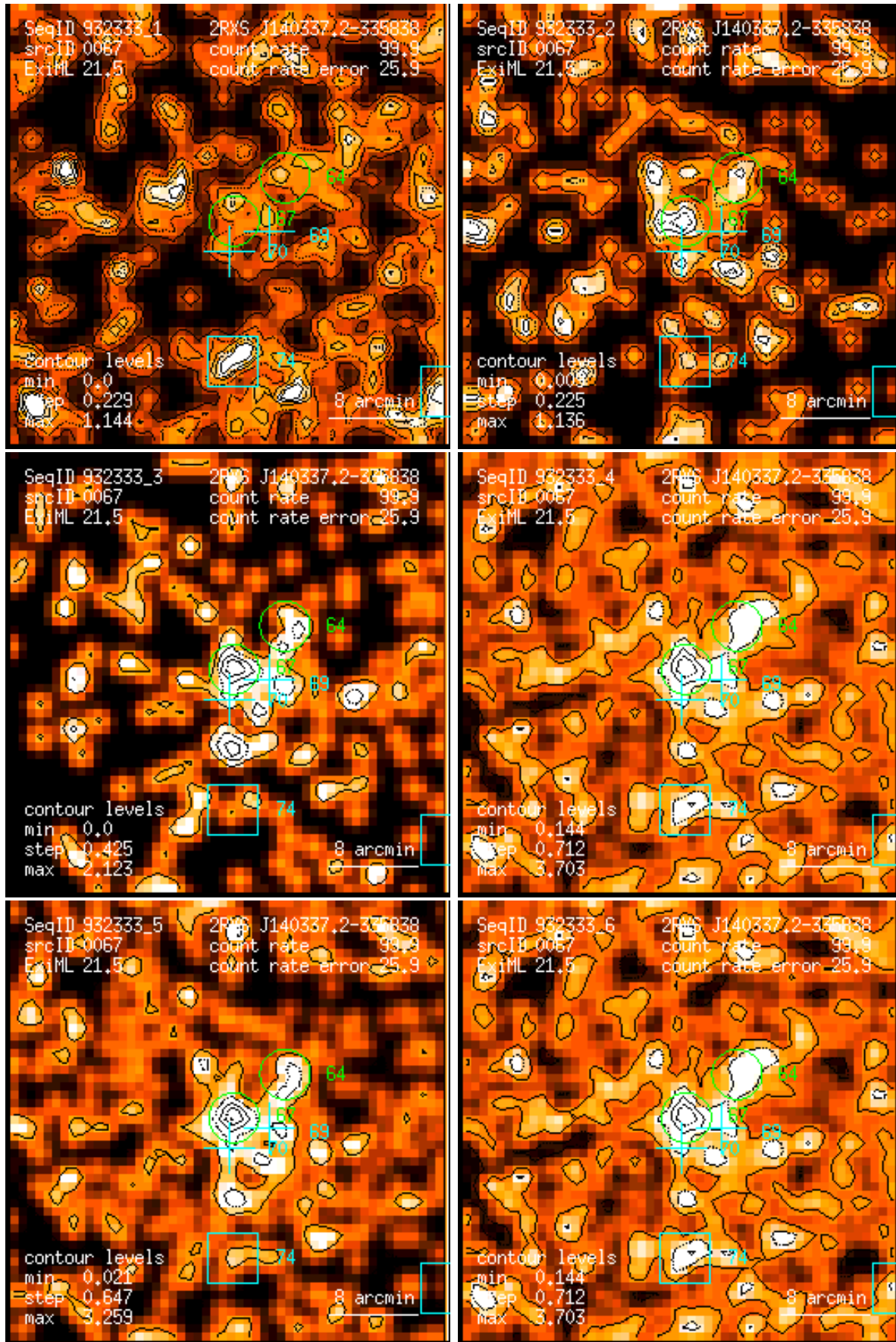
Figure 67: RASS 932333: detection 0067: band rate images, Gaussian filter: (1) PSPC channels 11 – 41, (2) 52 – 90, (3) 91 – 201, (4) 11 – 235, (5) 52 – 201, (6) 11 – 201. Broad band rates in counts/ks. Band rate contour levels in counts/ks/arcmin 2 .
