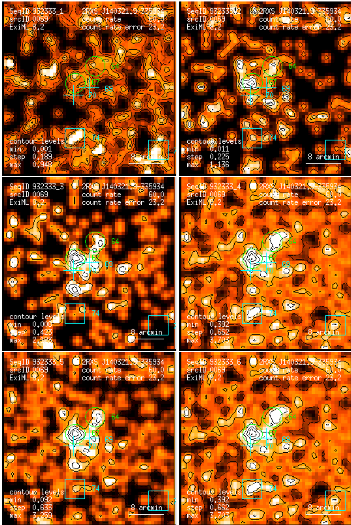
Figure 69: RASS 932333: detection 0069: band rate images, Gaussian filter: (1) PSPC channels 11 – 41, (2) 52 – 90, (3) 91 – 201, (4) 11 – 235, (5) 52 – 201, (6) 11 – 201. Broad band rates in counts/ks. Band rate contour levels in counts/ks/arcmin 2 .
