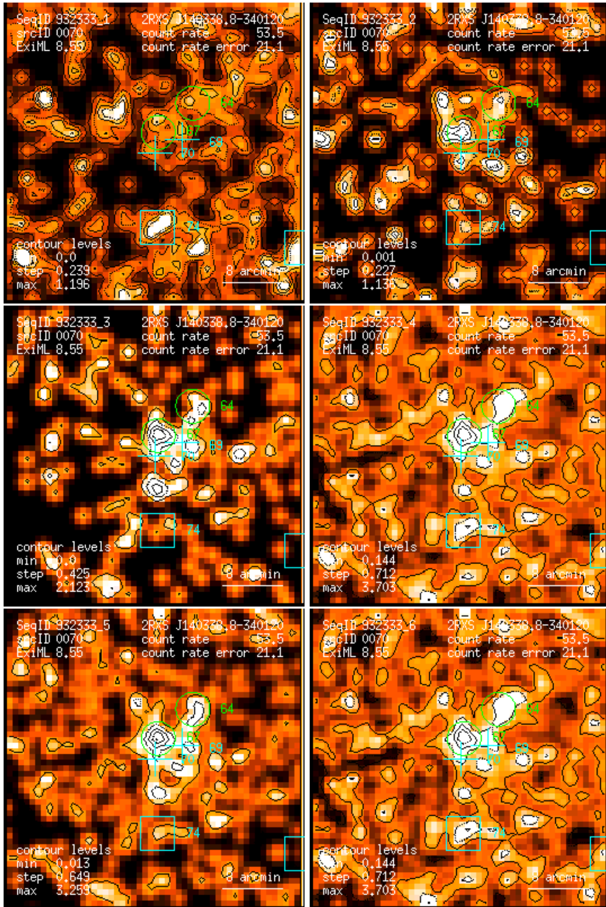
Figure 70: RASS 932333: detection 0070: band rate images, Gaussian filter: (1) PSPC channels 11 – 41, (2) 52 – 90, (3) 91 – 201, (4) 11 – 235, (5) 52 – 201, (6) 11 – 201. Broad band rates in counts/ks. Band rate contour levels in counts/ks/arcmin 2 .
