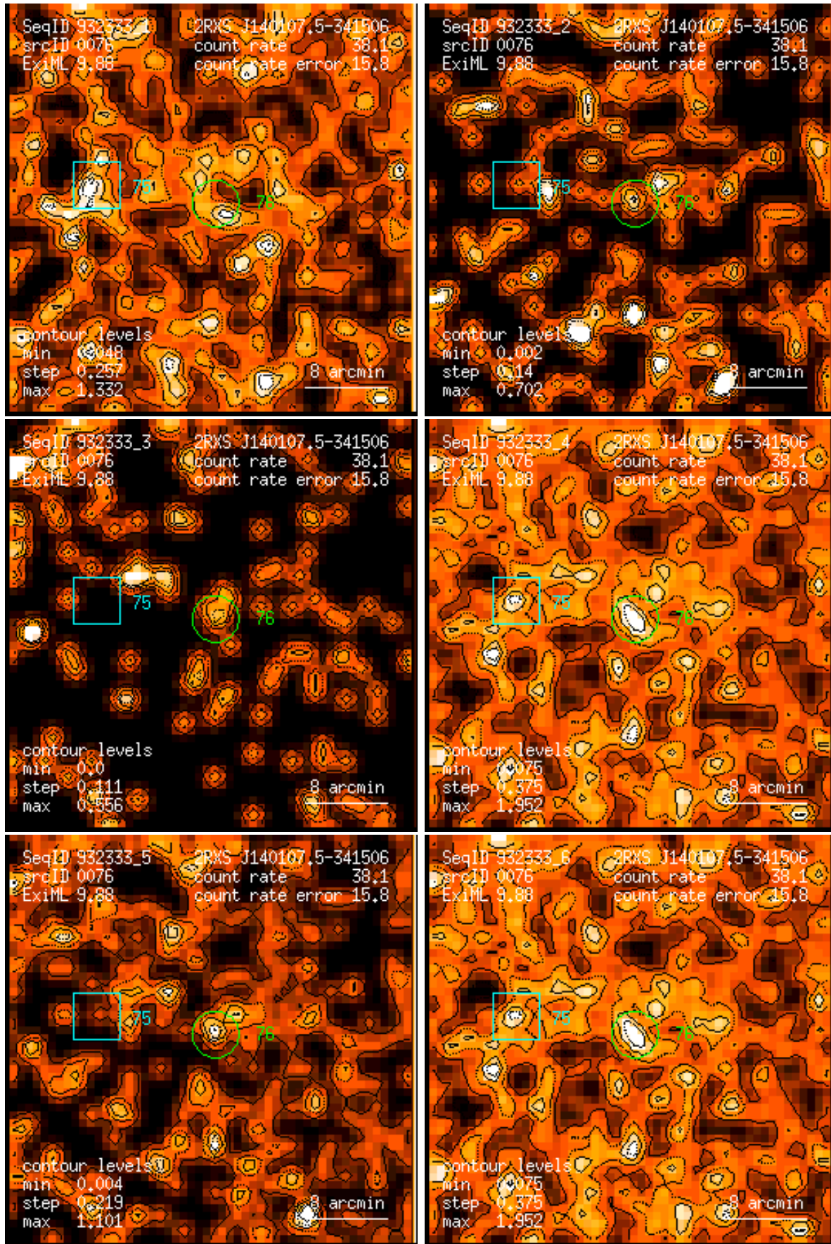
Figure 76: RASS 932333: detection 0076: band rate images, Gaussian filter: (1) PSPC channels 11 – 41, (2) 52 – 90, (3) 91 – 201, (4) 11 – 235, (5) 52 – 201, (6) 11 – 201. Broad band rates in counts/ks. Band rate contour levels in counts/ks/arcmin 2 .
