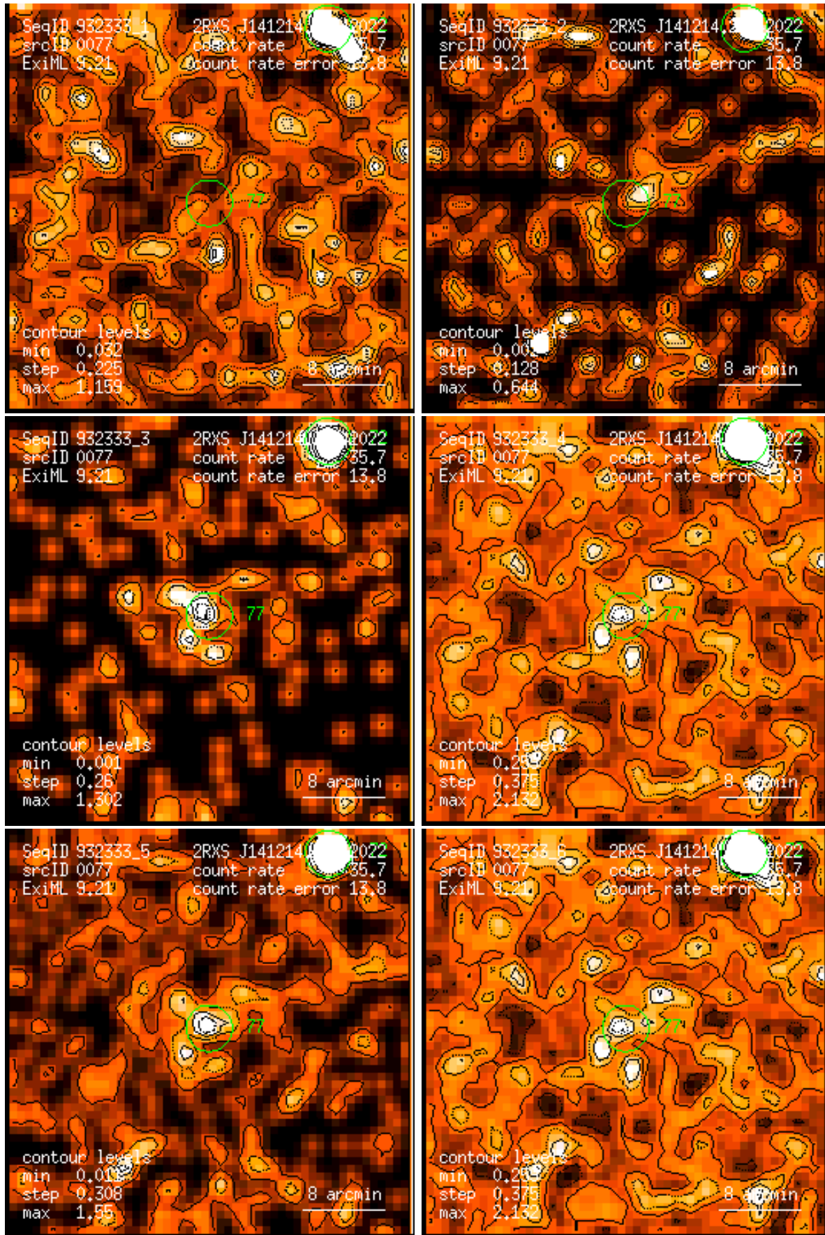
Figure 77: RASS 932333: detection 0077: band rate images, Gaussian filter: (1) PSPC channels 11 – 41, (2) 52 – 90, (3) 91 – 201, (4) 11 – 235, (5) 52 – 201, (6) 11 – 201. Broad band rates in counts/ks. Band rate contour levels in counts/ks/arcmin 2 .
