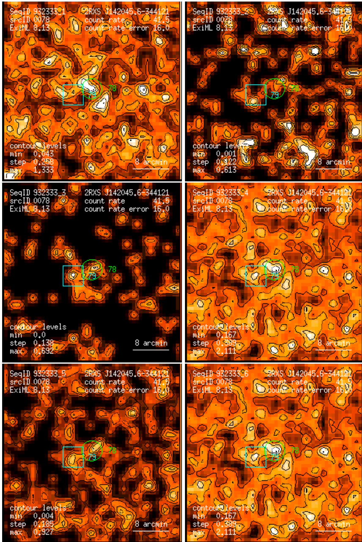
Figure 78: RASS 932333: detection 0078: band rate images, Gaussian filter: (1) PSPC channels 11 – 41, (2) 52 – 90, (3) 91 – 201, (4) 11 – 235, (5) 52 – 201, (6) 11 – 201. Broad band rates in counts/ks. Band rate contour levels in counts/ks/arcmin 2 .
