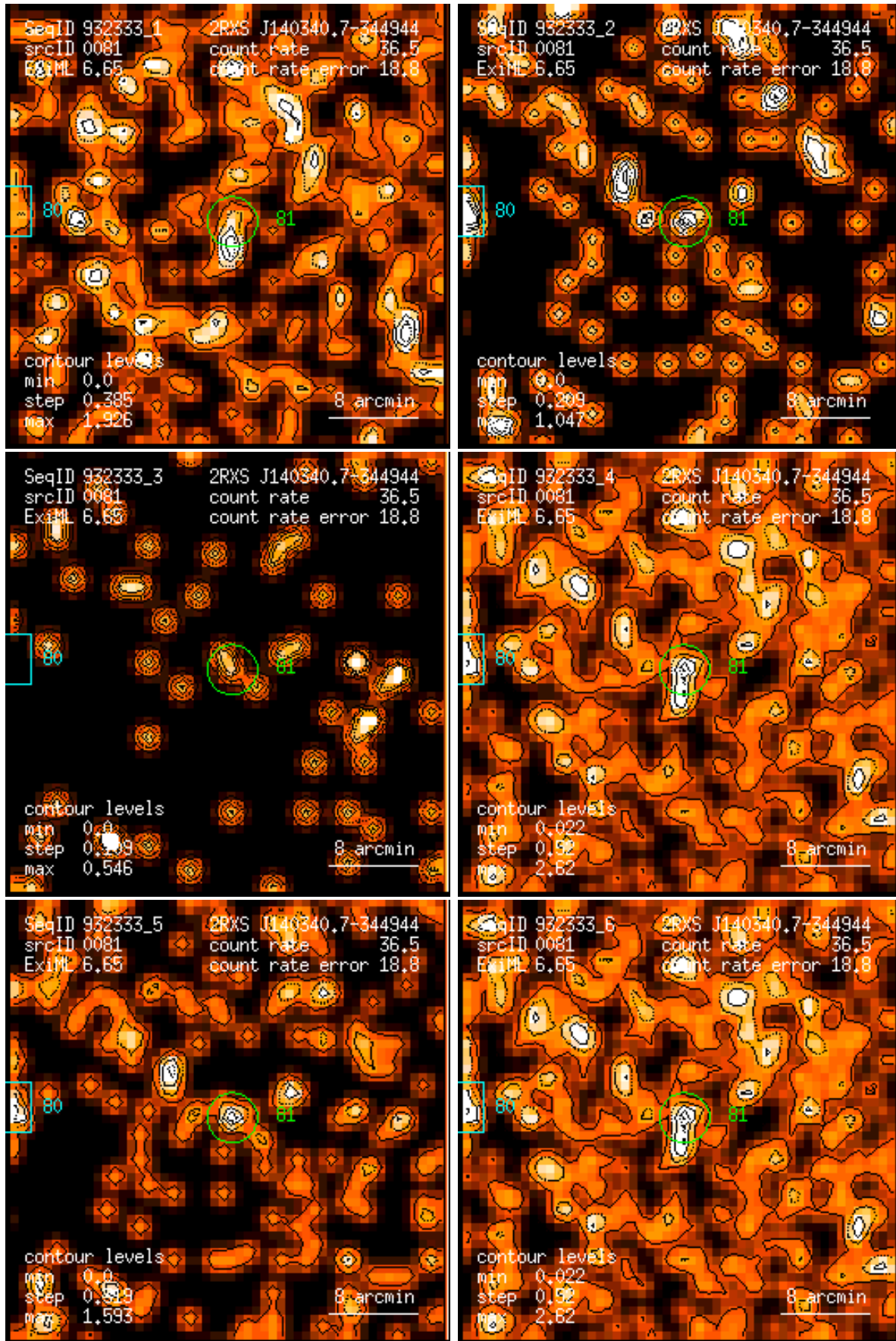
Figure 81: RASS 932333: detection 0081: band rate images, Gaussian filter: (1) PSPC channels 11 – 41, (2) 52 – 90, (3) 91 – 201, (4) 11 – 235, (5) 52 – 201, (6) 11 – 201. Broad band rates in counts/ks. Band rate contour levels in counts/ks/arcmin 2 .
