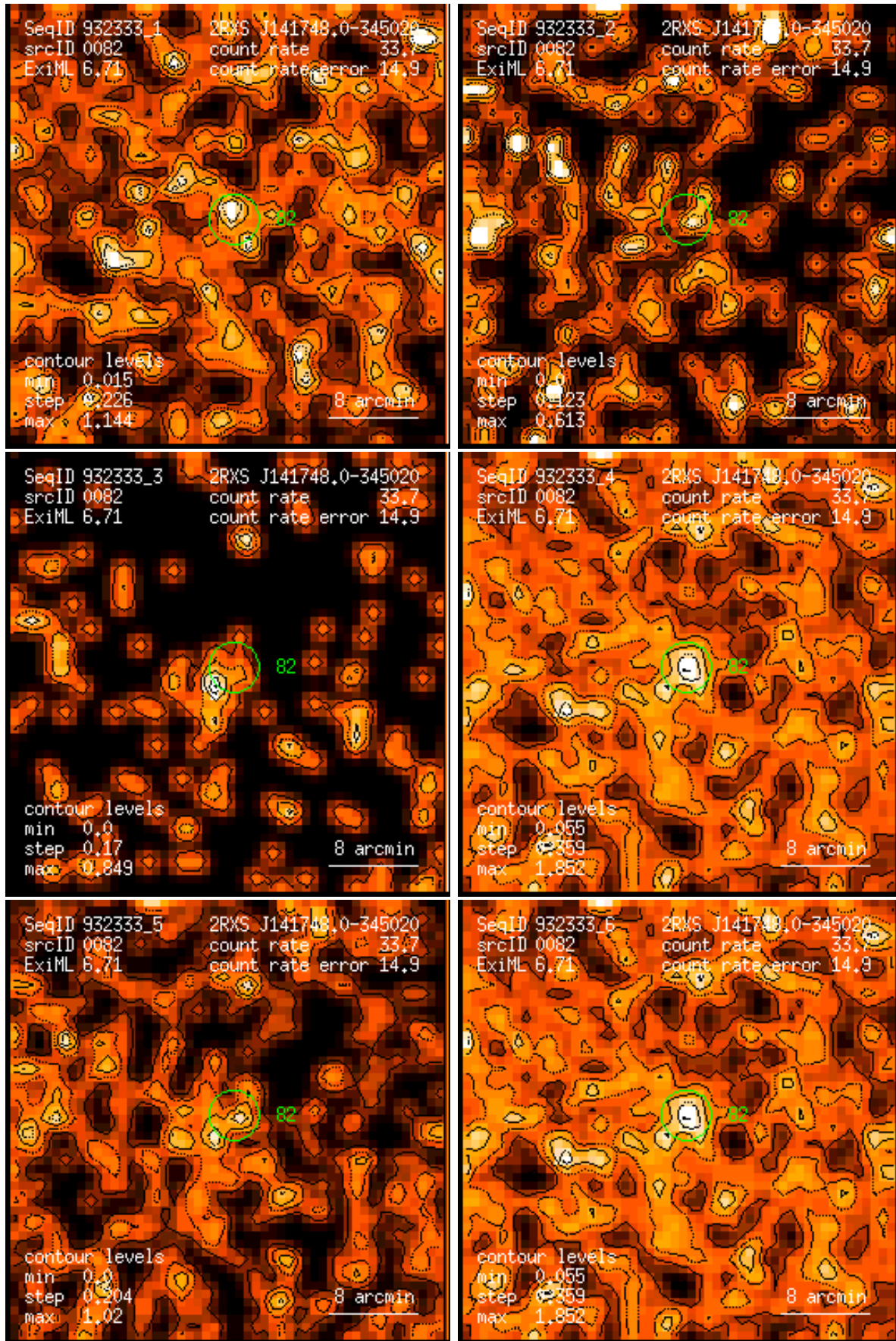
Figure 82: RASS 932333: detection 0082: band rate images, Gaussian filter: (1) PSPC channels 11 – 41, (2) 52 – 90, (3) 91 – 201, (4) 11 – 235, (5) 52 – 201, (6) 11 – 201. Broad band rates in counts/ks. Band rate contour levels in counts/ks/arcmin 2 .
