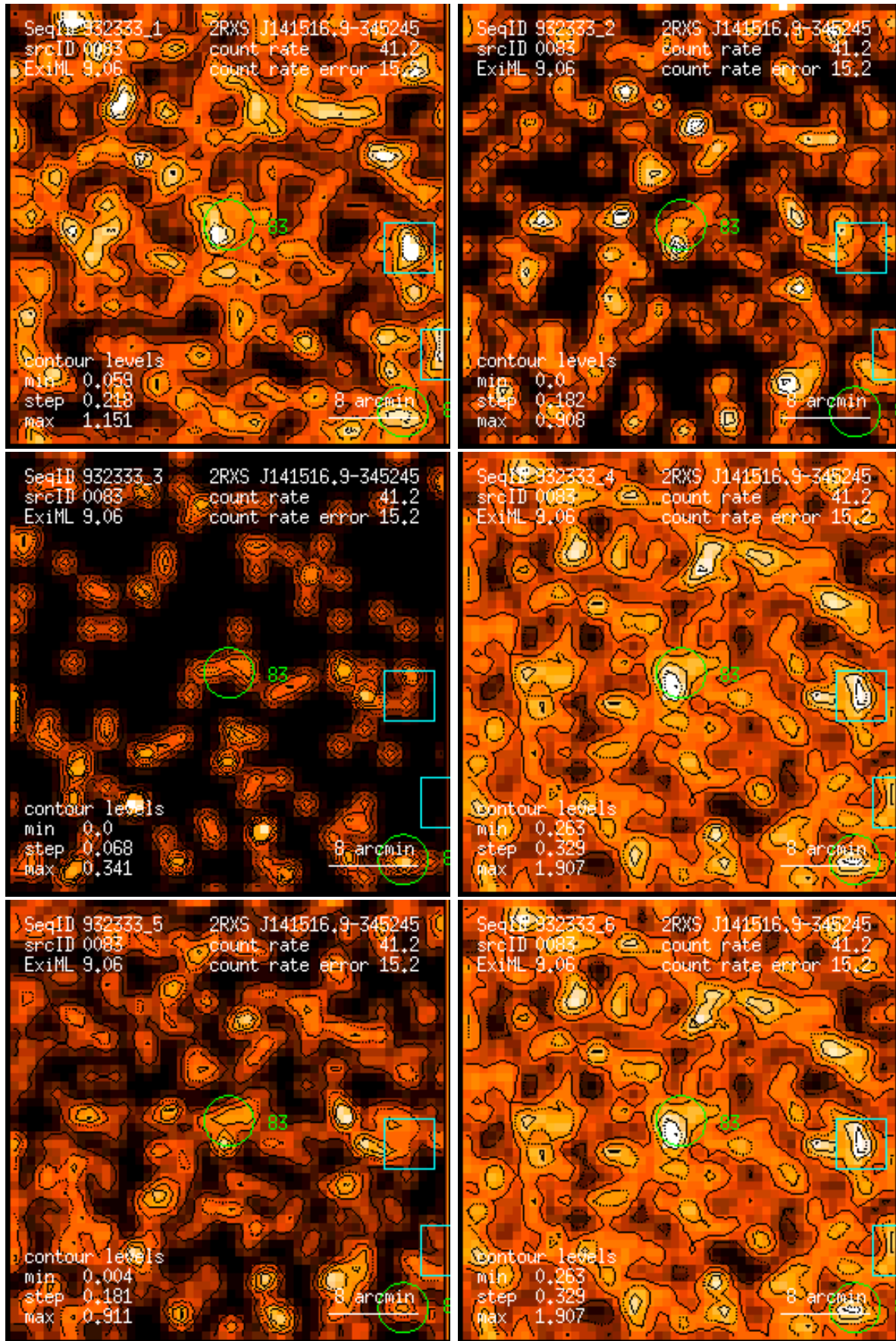
Figure 83: RASS 932333: detection 0083: band rate images, Gaussian filter: (1) PSPC channels 11 – 41, (2) 52 – 90, (3) 91 – 201, (4) 11 – 235, (5) 52 – 201, (6) 11 – 201. Broad band rates in counts/ks. Band rate contour levels in counts/ks/arcmin 2 .
