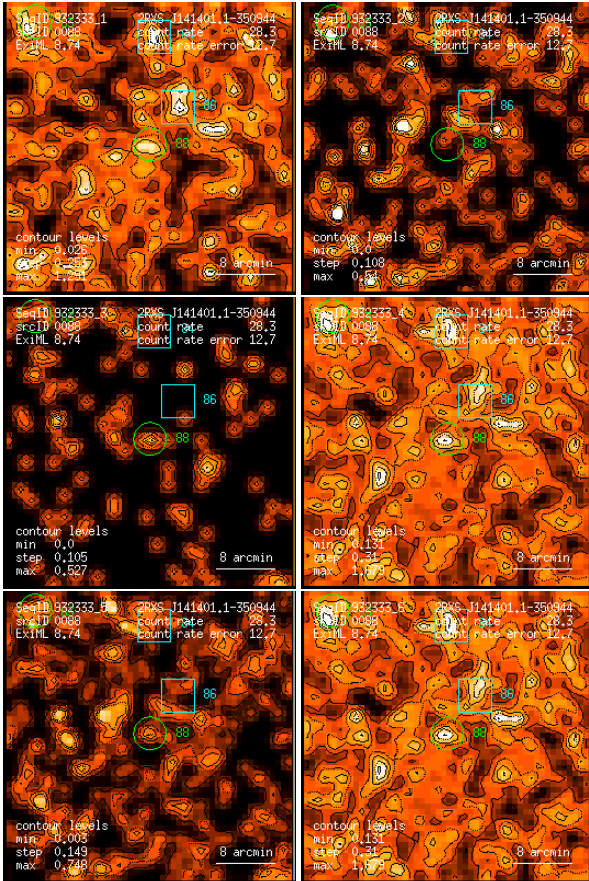
Figure 88: RASS 932333: detection 0088: band rate images, Gaussian filter: (1) PSPC channels 11 – 41, (2) 52 – 90, (3) 91 – 201, (4) 11 – 235, (5) 52 – 201, (6) 11 – 201. Broad band rates in counts/ks. Band rate contour levels in counts/ks/arcmin 2 .
