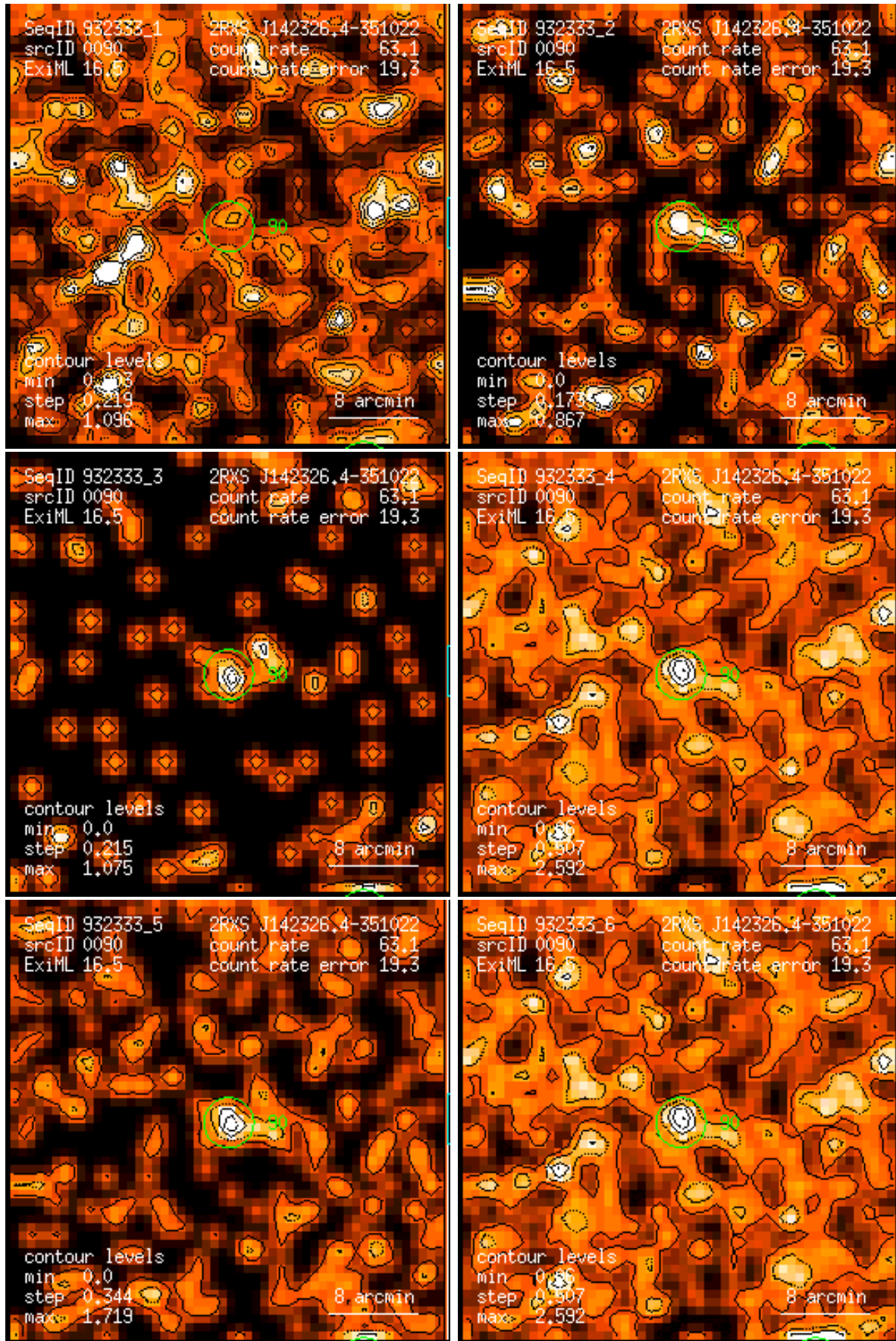
Figure 90: RASS 932333: detection 0090: band rate images, Gaussian filter: (1) PSPC channels 11 – 41, (2) 52 – 90, (3) 91 – 201, (4) 11 – 235, (5) 52 – 201, (6) 11 – 201. Broad band rates in counts/ks. Band rate contour levels in counts/ks/arcmin 2 .
