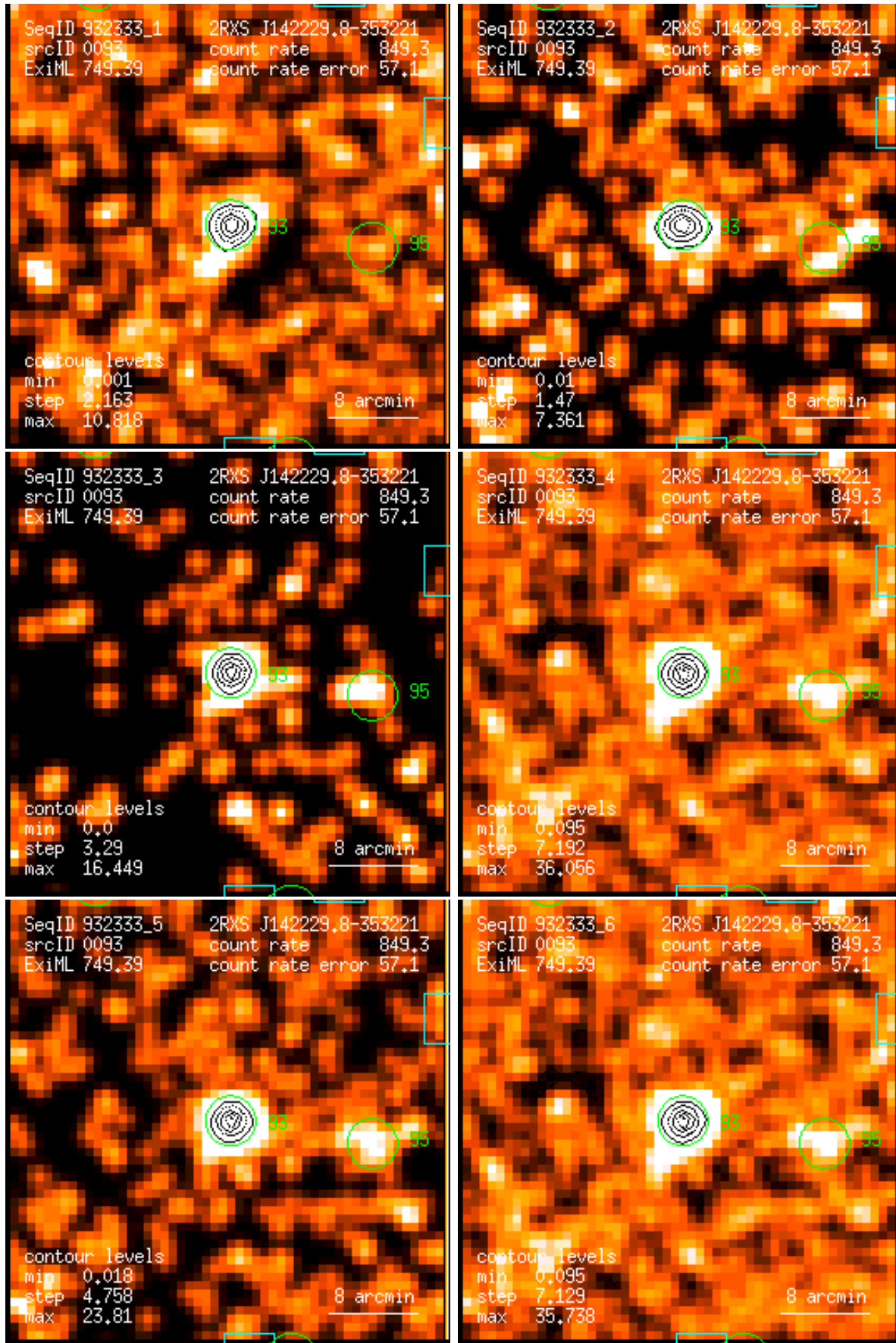
Figure 93: RASS 932333: detection 0093: band rate images, Gaussian filter: (1) PSPC channels 11 – 41, (2) 52 – 90, (3) 91 – 201, (4) 11 – 235, (5) 52 – 201, (6) 11 – 201. Broad band rates in counts/ks. Band rate contour levels in counts/ks/arcmin 2 .
