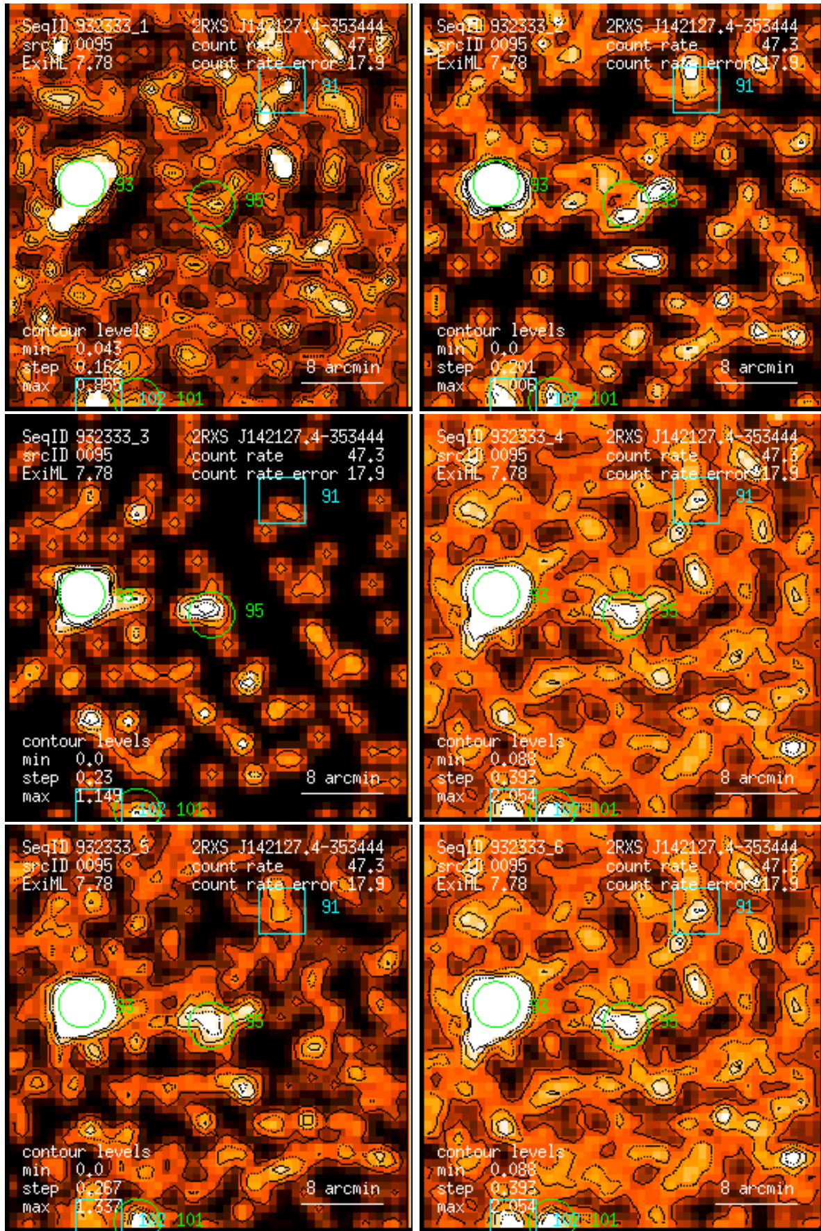
Figure 95: RASS 932333: detection 0095: band rate images, Gaussian filter: (1) PSPC channels 11 – 41, (2) 52 – 90, (3) 91 – 201, (4) 11 – 235, (5) 52 – 201, (6) 11 – 201. Broad band rates in counts/ks. Band rate contour levels in counts/ks/arcmin 2 .
