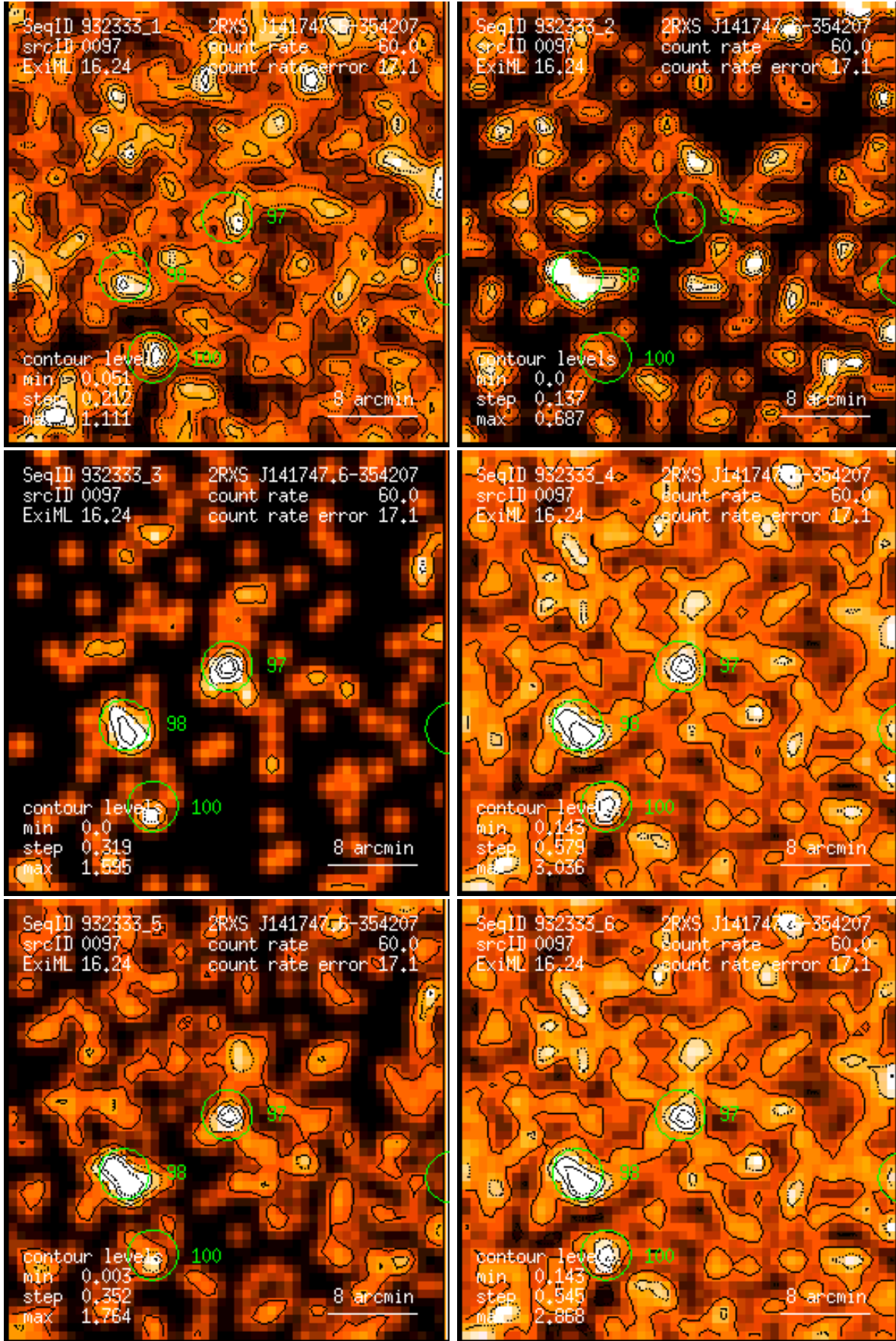
Figure 97: RASS 932333: detection 0097: band rate images, Gaussian filter: (1) PSPC channels 11 – 41, (2) 52 – 90, (3) 91 – 201, (4) 11 – 235, (5) 52 – 201, (6) 11 – 201. Broad band rates in counts/ks. Band rate contour levels in counts/ks/arcmin 2 .
