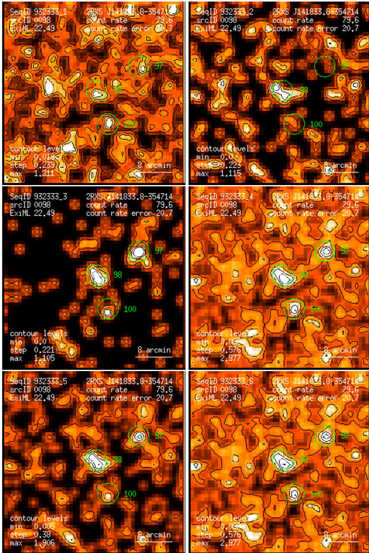
Figure 98: RASS 932333: detection 0098: band rate images, Gaussian filter: (1) PSPC channels 11 – 41, (2) 52 – 90, (3) 91 – 201, (4) 11 – 235, (5) 52 – 201, (6) 11 – 201. Broad band rates in counts/ks. Band rate contour levels in counts/ks/arcmin 2 .
