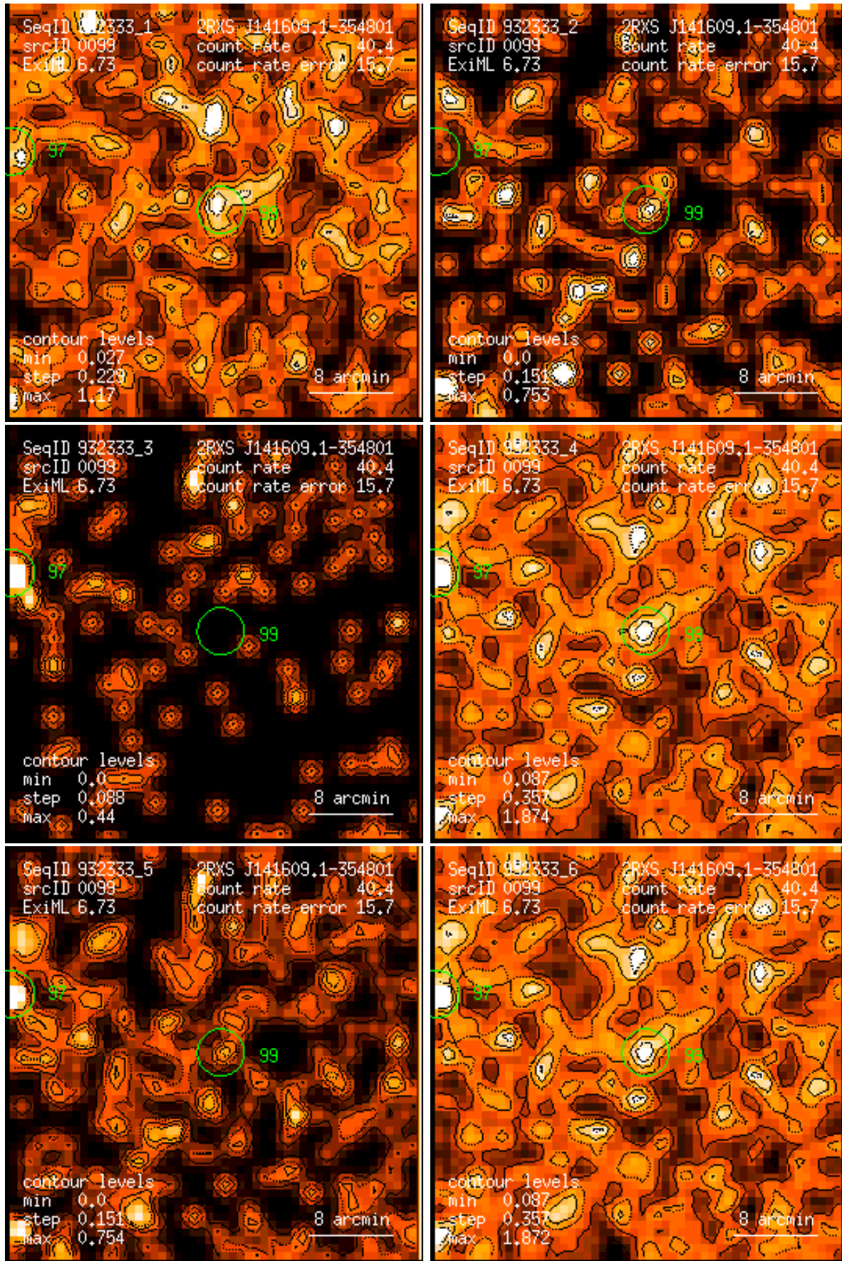
Figure 99: RASS 932333: detection 0099: band rate images, Gaussian filter: (1) PSPC channels 11 – 41, (2) 52 – 90, (3) 91 – 201, (4) 11 – 235, (5) 52 – 201, (6) 11 – 201. Broad band rates in counts/ks. Band rate contour levels in counts/ks/arcmin 2 .
