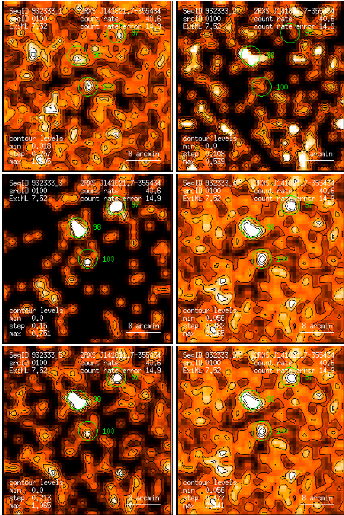
Figure 100: RASS 932333: detection 0100: band rate images, Gaussian filter: (1) PSPC channels 11 – 41, (2) 52 – 90, (3) 91 – 201, (4) 11 – 235, (5) 52 – 201, (6) 11 – 201. Broad band rates in counts/ks. Band rate contour levels in counts/ks/arcmin 2 .
