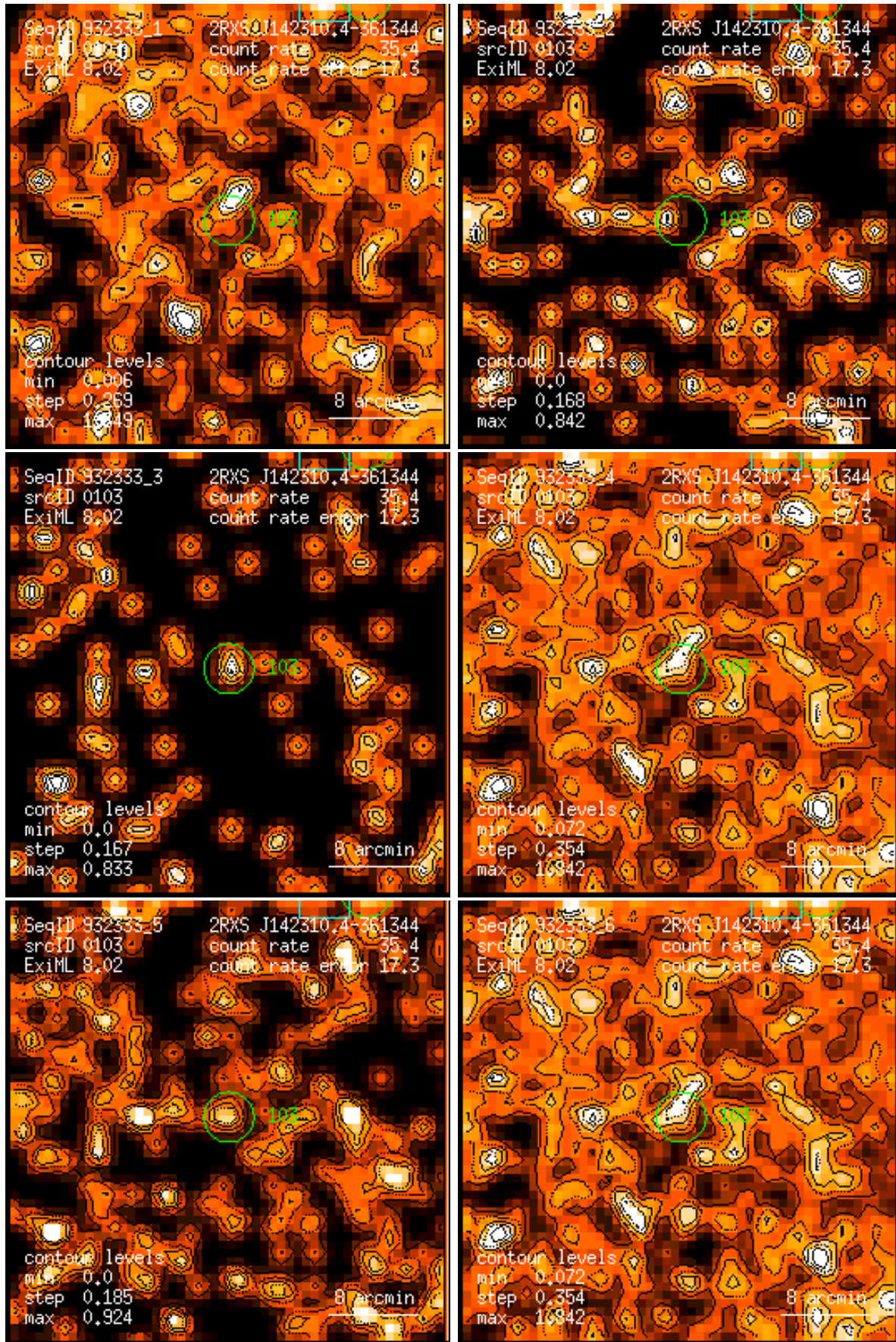
Figure 103: RASS 932333: detection 0103: band rate images, Gaussian filter: (1) PSPC channels 11 – 41, (2) 52 – 90, (3) 91 – 201, (4) 11 – 235, (5) 52 – 201, (6) 11 – 201. Broad band rates in counts/ks. Band rate contour levels in counts/ks/arcmin 2 .
