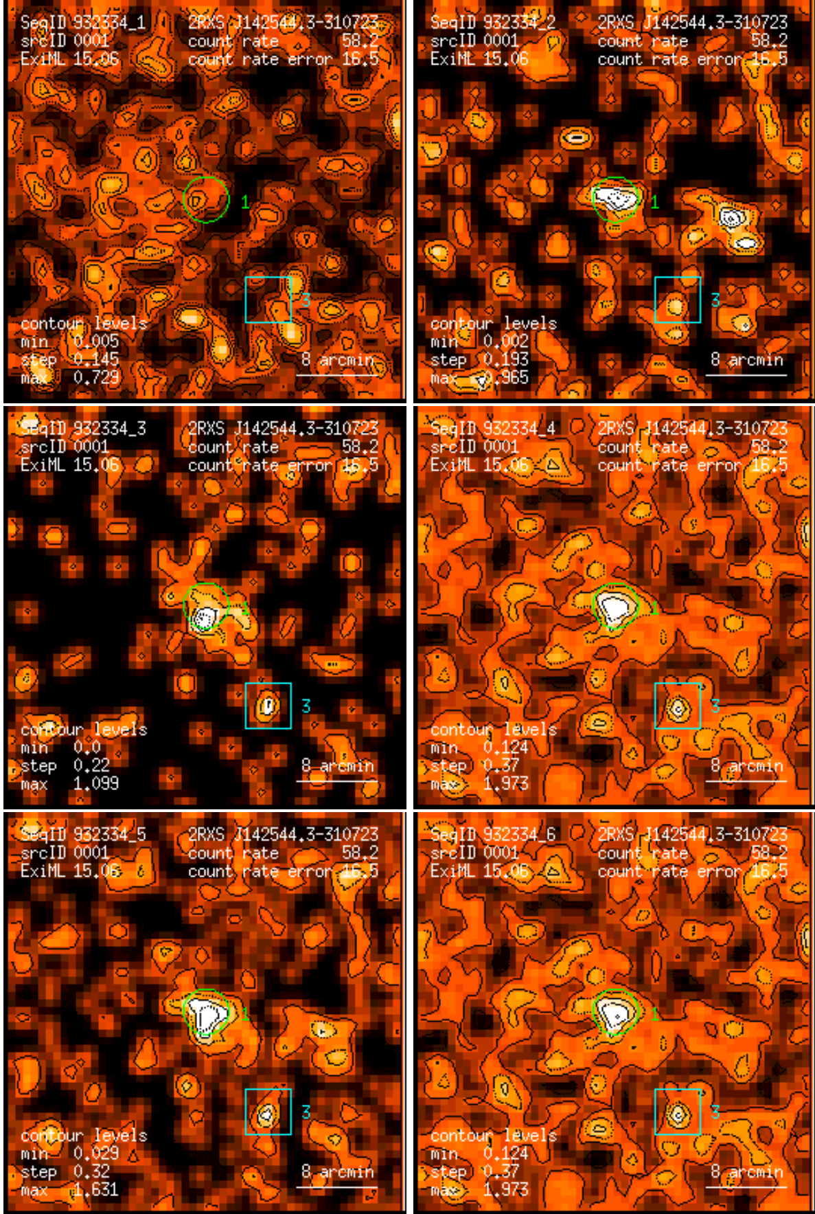
Figure 1: RASS 932334: detection 0001: band rate images, Gaussian filter: (1) PSPC channels 11 – 41, (2) 52 – 90, (3) 91 – 201, (4) 11 – 235, (5) 52 – 201, (6) 11 – 201. Broad band rates in counts/ks. Band rate contour levels in counts/ks/arcmin 2 .
