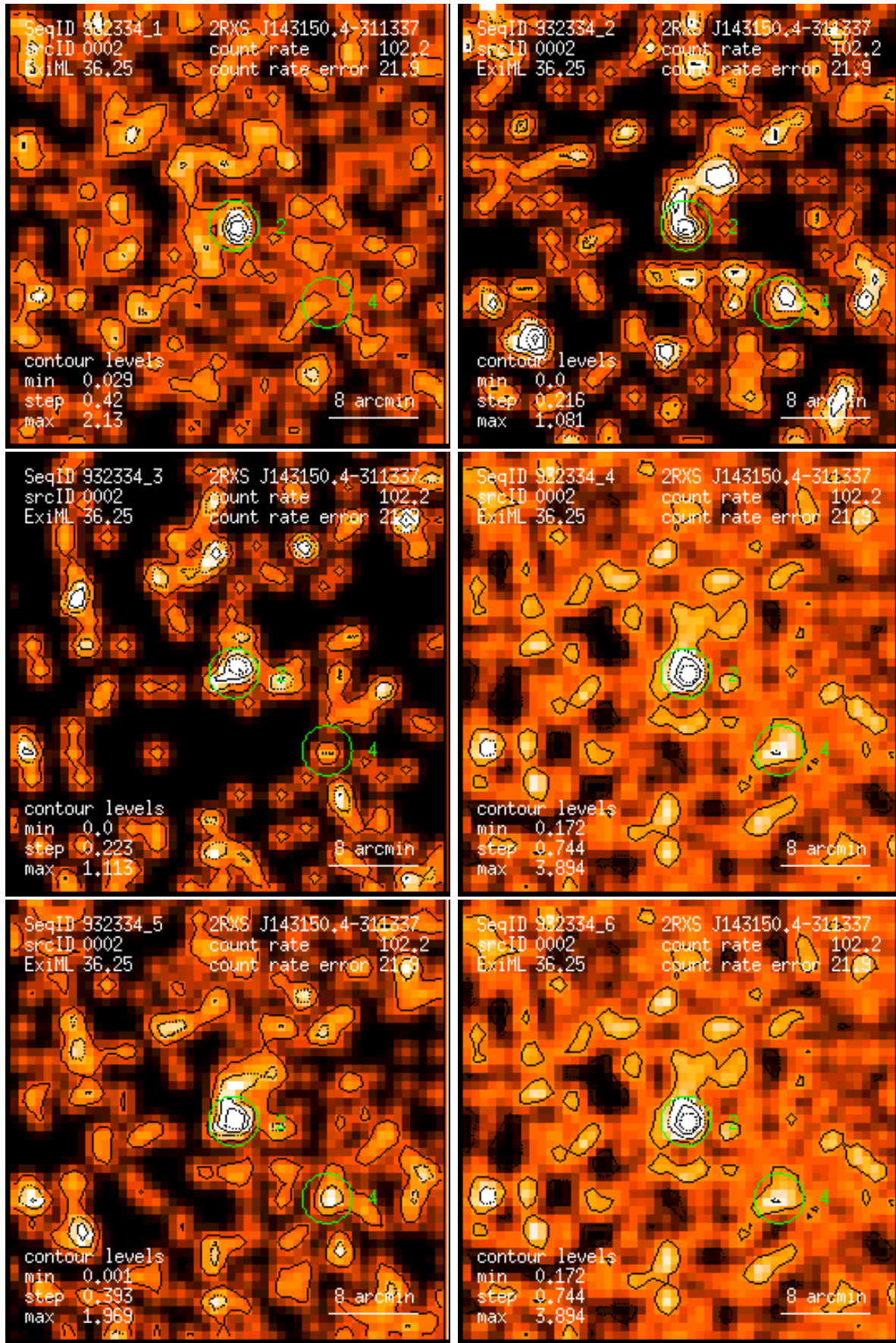
Figure 2: RASS 932334: detection 0002: band rate images, Gaussian filter: (1) PSPC channels 11 – 41, (2) 52 – 90, (3) 91 – 201, (4) 11 – 235, (5) 52 – 201, (6) 11 – 201. Broad band rates in counts/ks. Band rate contour levels in counts/ks/arcmin 2 .
