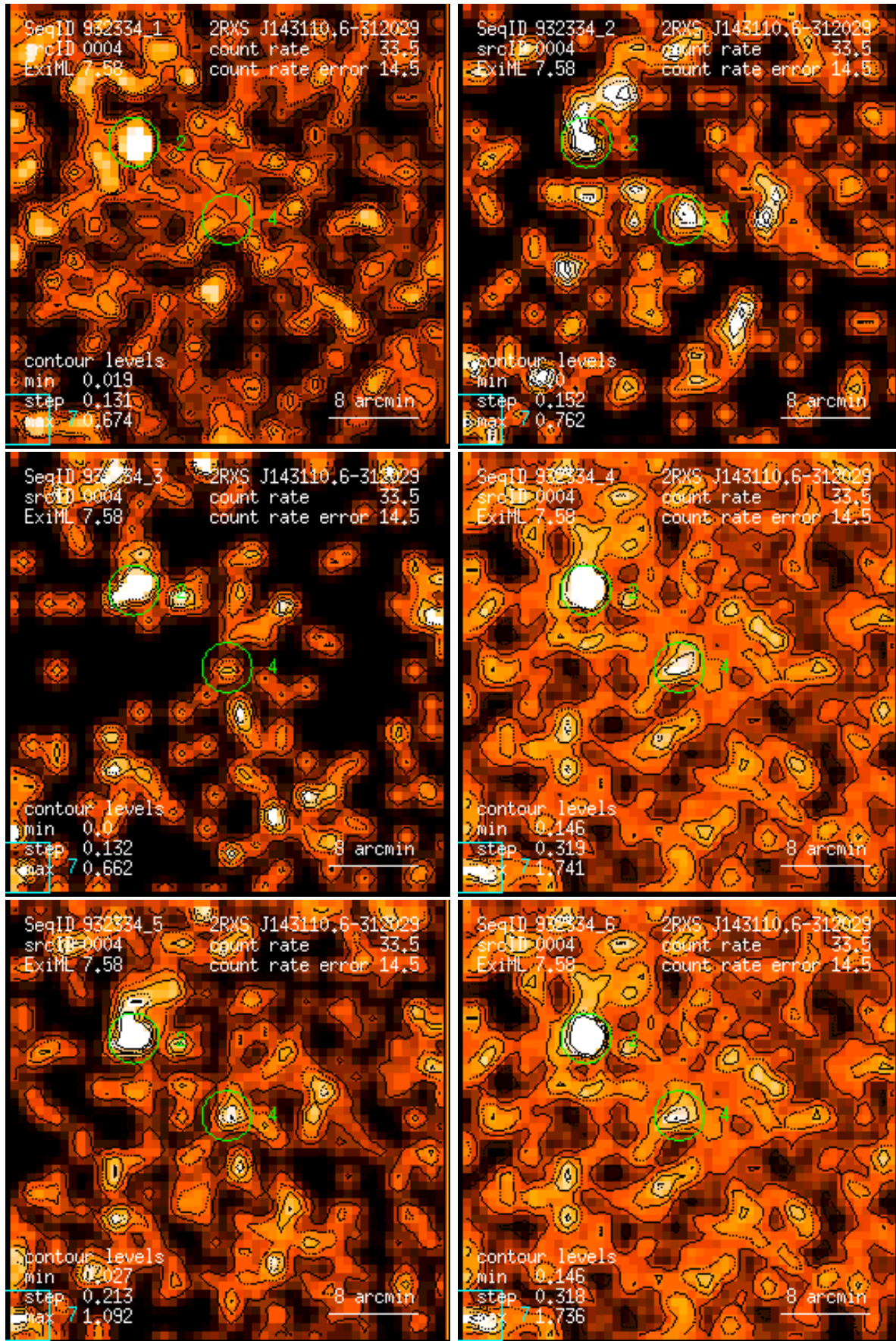
Figure 4: RASS 932334: detection 0004: band rate images, Gaussian filter: (1) PSPC channels 11 – 41, (2) 52 – 90, (3) 91 – 201, (4) 11 – 235, (5) 52 – 201, (6) 11 – 201. Broad band rates in counts/ks. Band rate contour levels in counts/ks/arcmin 2 .
