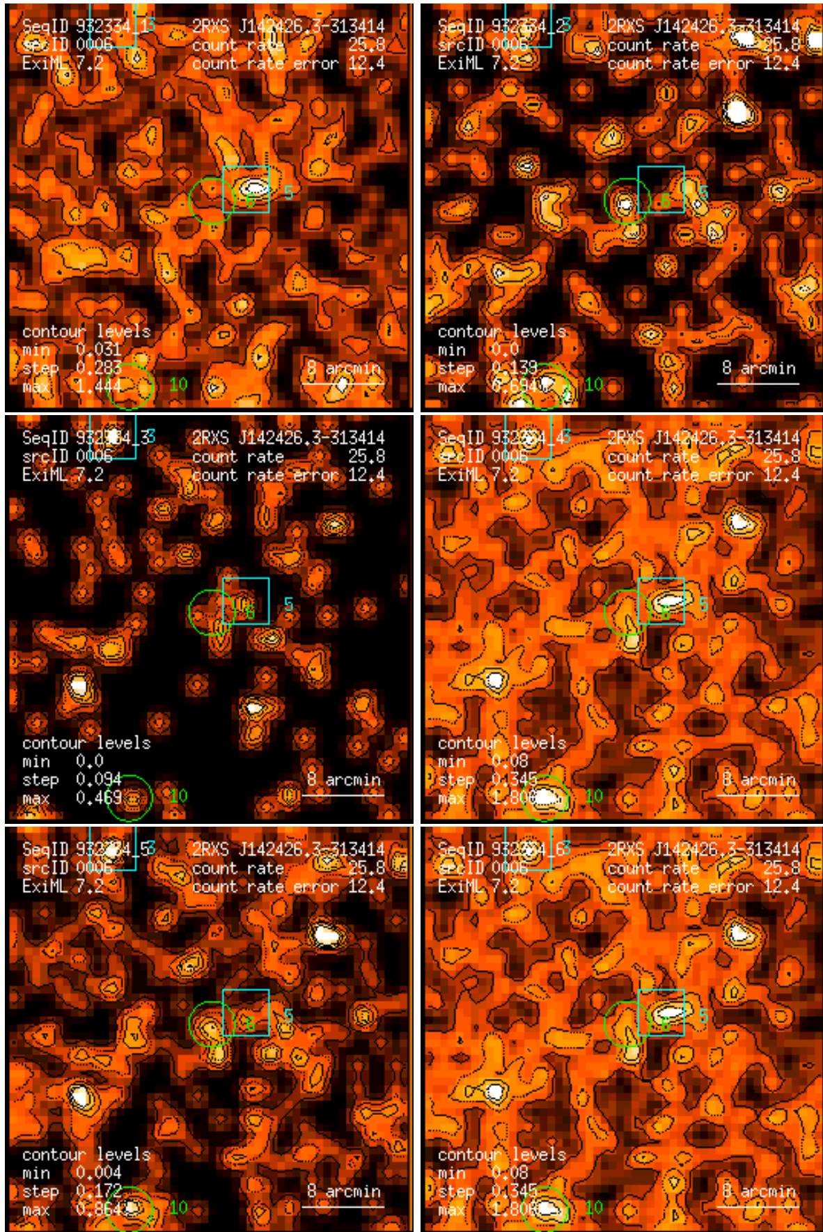
Figure 6: RASS 932334: detection 0006: band rate images, Gaussian filter: (1) PSPC channels 11 – 41, (2) 52 – 90, (3) 91 – 201, (4) 11 – 235, (5) 52 – 201, (6) 11 – 201. Broad band rates in counts/ks. Band rate contour levels in counts/ks/arcmin 2 .
